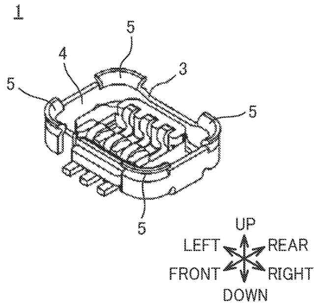
FIG. 17 PRIOR ART
