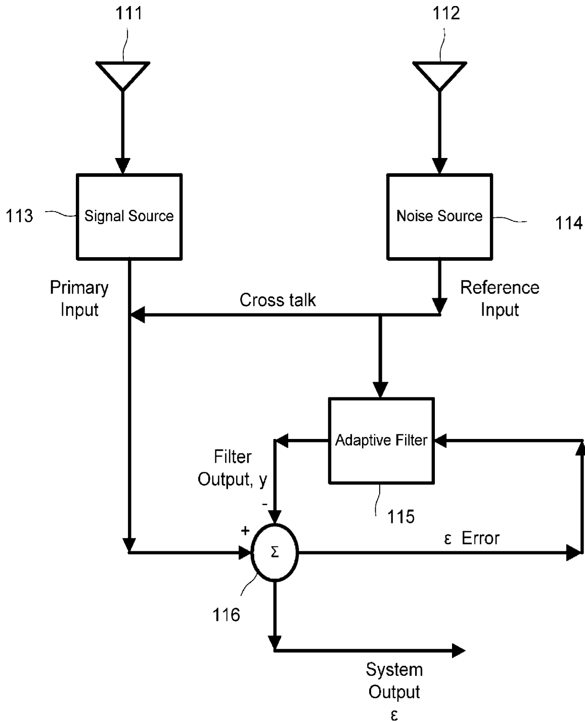
FIG. 1 PRIOR ART
