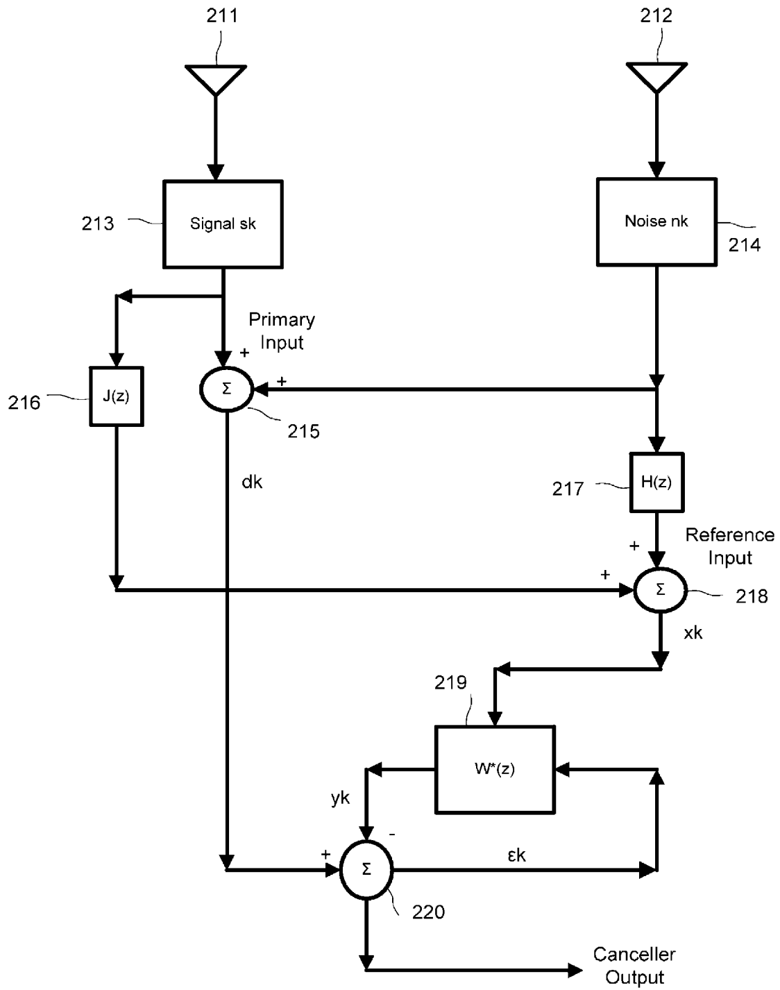
FIG. 2 PRIOR ART
