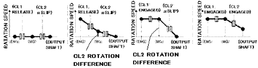
FIG. 5 ROTATION SPEED RELATIONSHIP AT VEHICLE STOPPED STATE
