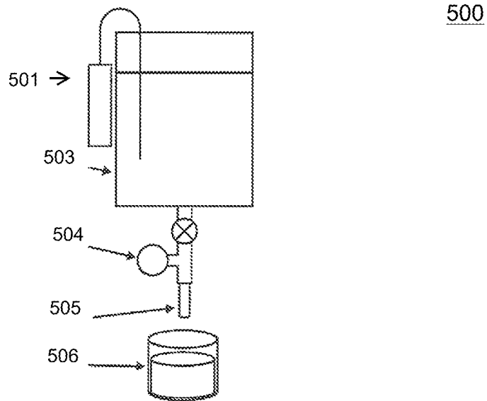
Hydraulic Resistance Characterization Fixture
