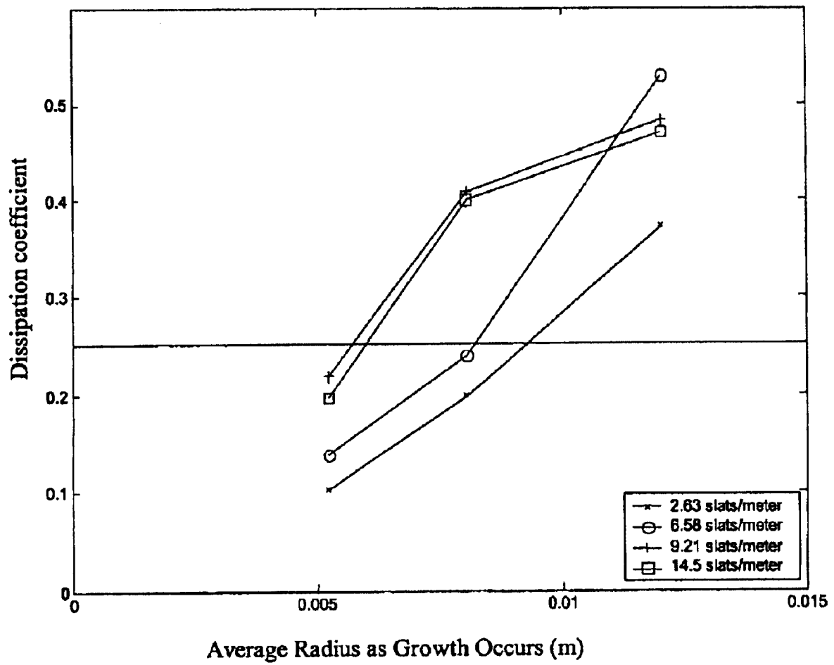
The effects of growth on wave dissipation: Wave Type 1
