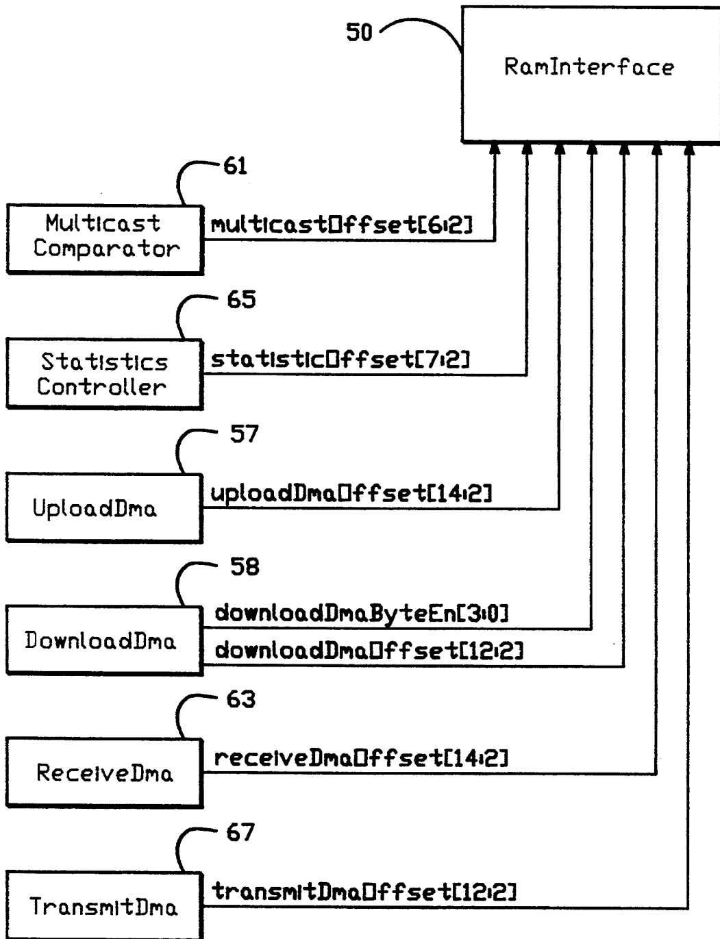
Autonomous Access Address Bus Structure
