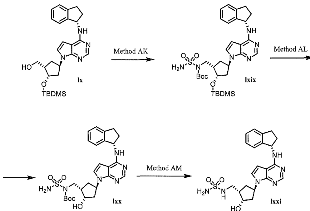
Scheme 13: General route to 4-substituted ((1 S ,2 S ,4 R )-2-hydroxy-4-{7 H -pyrrolo[2,3- d ]pyrimidin-7-yl}cyclopentyl)methyl sulfamides
