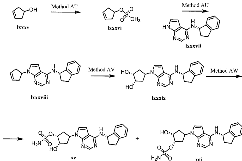
Scheme 16: Synthesis of Diastereoisomeric mixture of (1 S ,2 R ,4 R )-4-[4-[(1 S )-2,3-dihydro-1 H -inden-1-ylamino]-7 H -pyrrolo[2,3- d ]pyrimidin-7-yl]-2-hydroxycyclopentyl sulfamate and (1 R ,2 S ,4 S )-4-[4-[(1 S )-2,3-dihydro-1 H -inden-1-ylamino]-7 H -pyrrolo[2,3- d ]pyrimidin-7-yl]-2-hydroxycyclopentyl sulfamate
