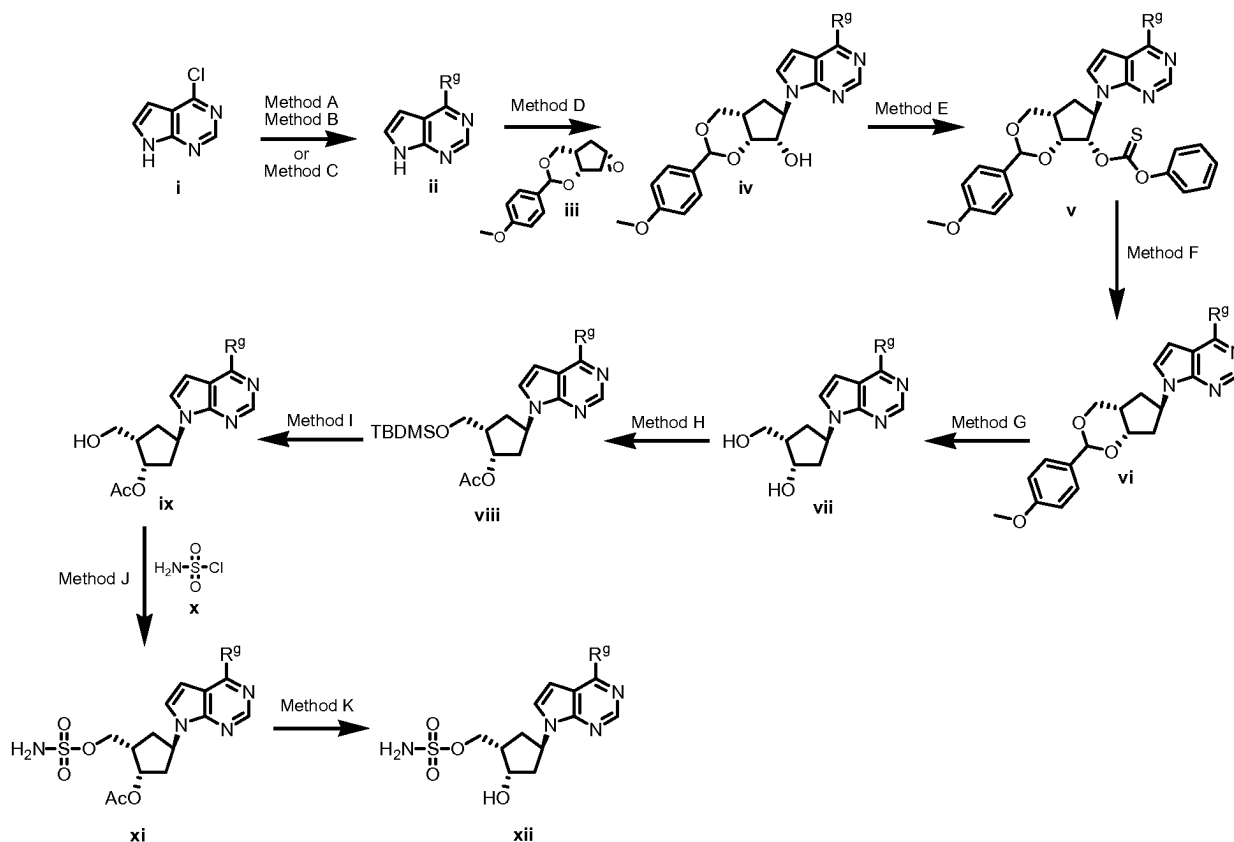
Scheme 1: General route for the synthesis of 4-substituted ((1 S ,2 S ,4 R )-2-hydroxy-4-{7 H -pyrrolo[2,3- d ]pyrimidin-7-yl}cyclopentyl)methyl sulfamates
