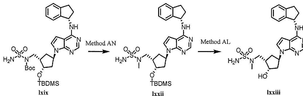
Scheme 14: General route to 4-substituted ((1 S ,2 S ,4 R )-2-hydroxy-4-{7 H -pyrrolo[2,3- d ]-pyrimidin-7-yl)cyclopentyl)methyl N -methyl sulfamides
