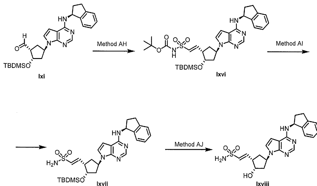
Scheme 12: Synthesis of ( E )-2-((1 S ,2 S ,4 R )-4-[4-[(1 S )-2,3-dihydro-1 H -inden-1-ylamino]-7 H -pyrrolo[2,3- d ]pyrimidin-7-yl]-2-hydroxycyclopentyl)ethanesulfonamide
