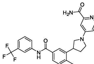
Example 55 (Second eluting)
