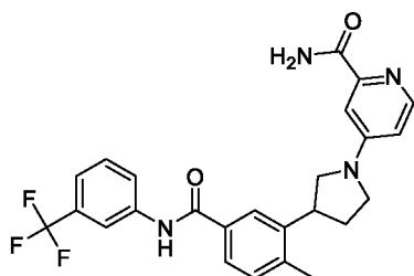
Example 54 (First eluting)
