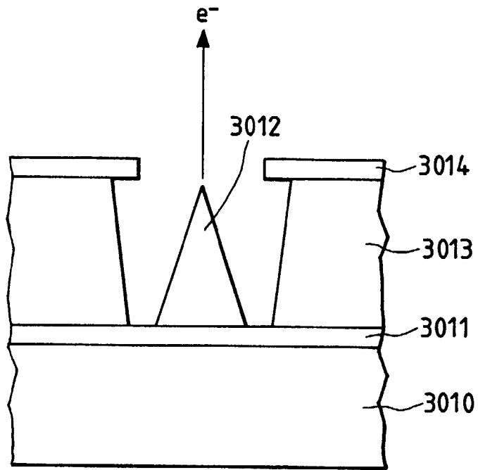
FIG. 37 PRIOR ART
