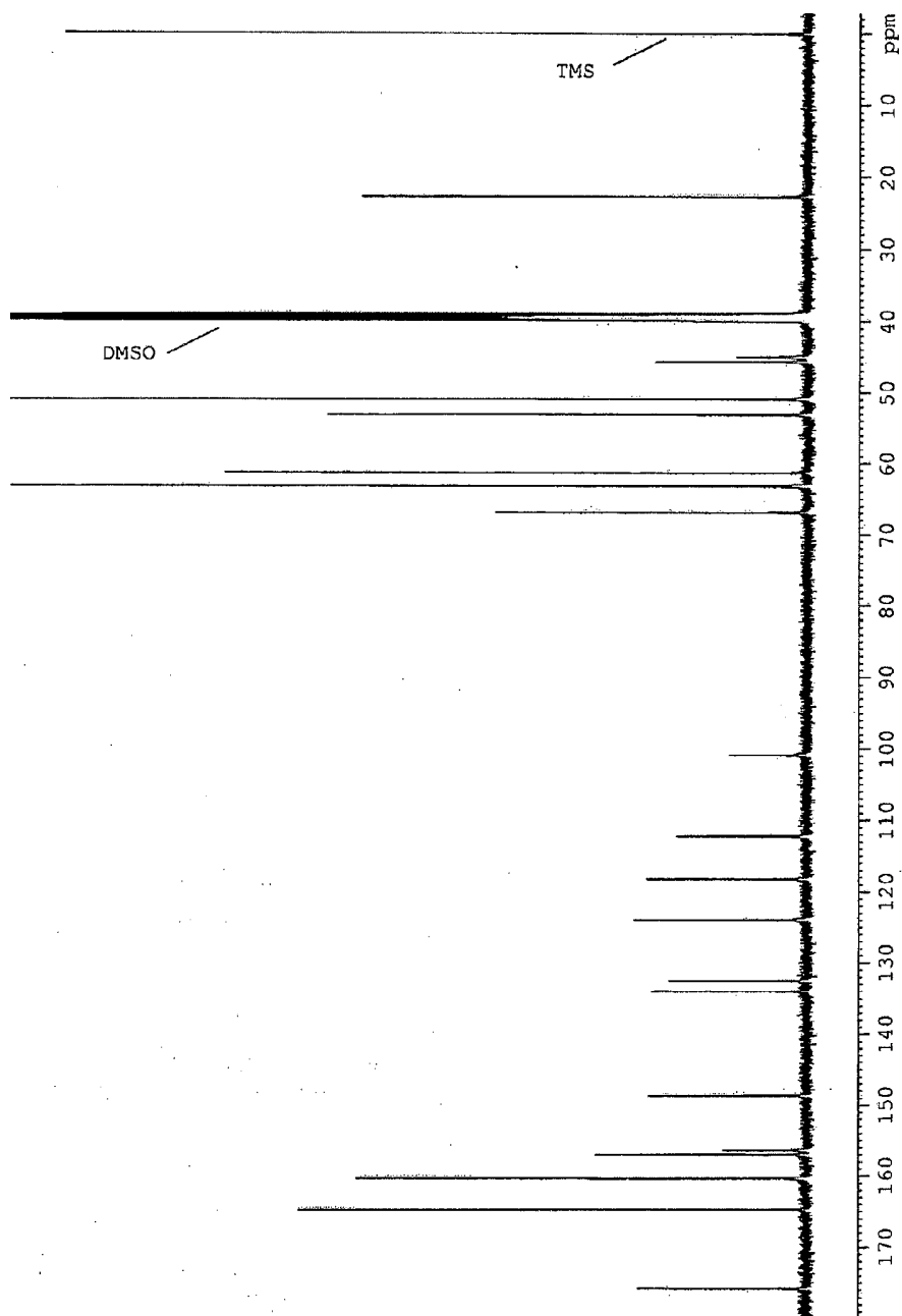
FIGURE 5 13 C-NMR Spectrum of the dihydrochloride of formula (II)
