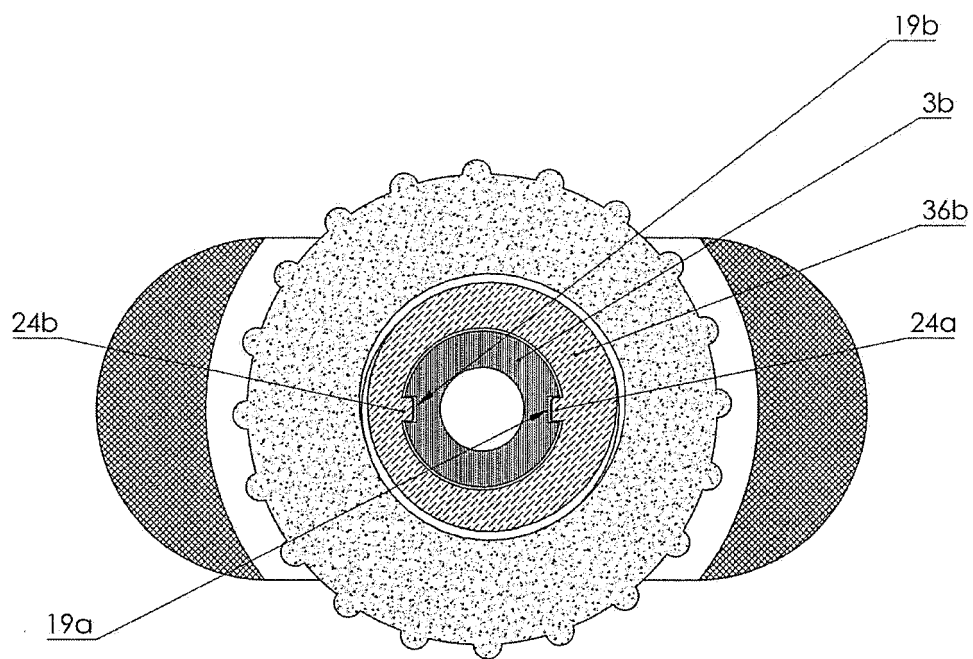
CROSS-SECTION D-D
