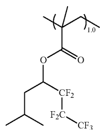
Water-repellent polymer 1 Mw = 8,900 Mw/Mn = 1.96
