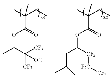
Water-repellent polymer 2 Mw = 9,300 Mw/Mn = 1.87
