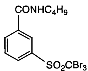
Organic polyhalogen compound-2
