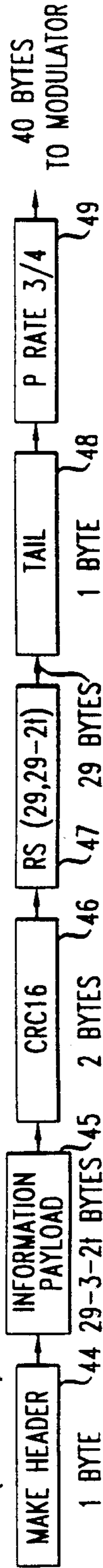
FIG. 2F P+RS (29,29-2t): PUNCTURED CONVOLUTION CODE WITH 1-ERROR CORRECTING RS
