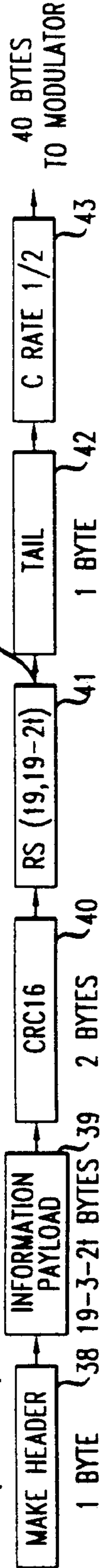
FIG. 2E C+RS (19,19-2t): FULL CONVOLUTION CODE WITH 1-ERROR CORRECTING RS
