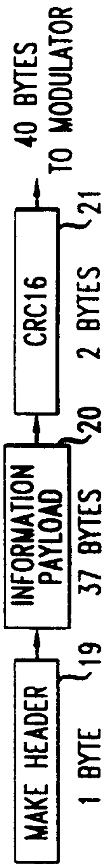
FIG. 2A U: UNCODED
