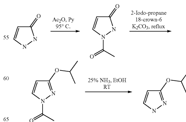
Scheme 1e Preparation of intermediate 3-isopropoxy-1H-pyrazole for preparing e.g., Example 1b-151
