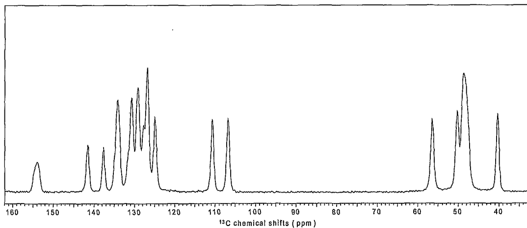
Figure 4: 13 C solid state NMR spectrum of polymorphic form \alpha of bifeprunox mesilate
