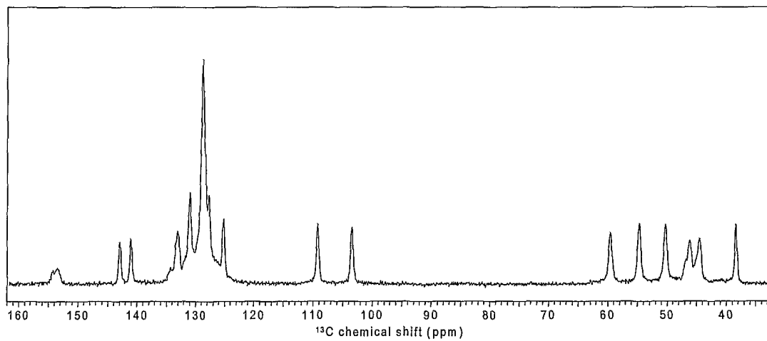
Figure 9: 13 C solid state NMR spectrum of polymorphic form \gamma of bifeprunox mesilate
