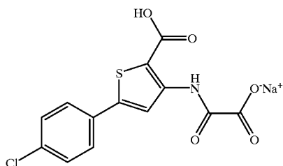
5-(4-Chloro-phenyl)-3-(oxalyl-amino)-thiophene-2-carboxylic acid, mono sodium salt
