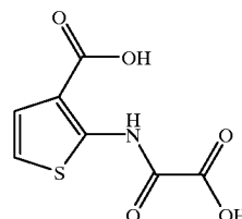
2-(Oxalyl-amino)-thiophene-3-carboxylic acid
