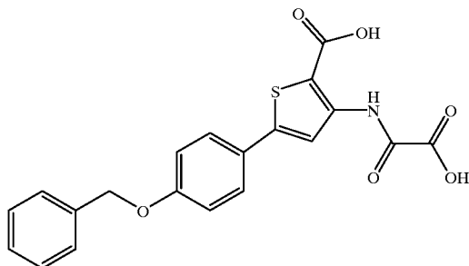
5-(4-Benzoyloxy-phenyl)-3-(oxalyl-amino)-thiophene-2-carboxylic acid
