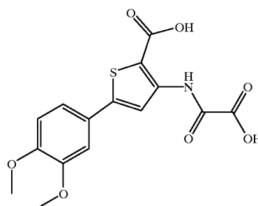
5-(3,4-Dimethoxy-phenyl)-3-(oxalyl-amino)-thiophene-2-carboxylic acid
