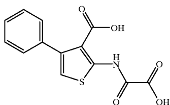
2-(Oxalyl-amino)-4-phenyl-thiophene-3-carboxylic acid
