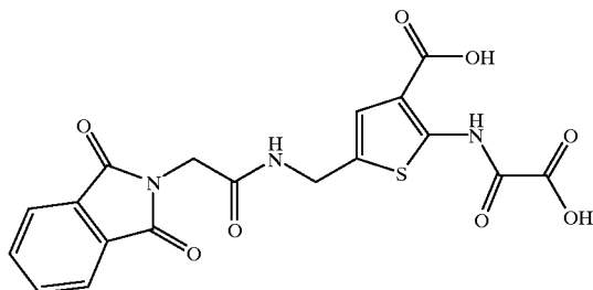
5-((2-(1,3-Dioxo-1,3-dihydro-isoindol-2-yl)-acetyl-amino)-methyl)-2-(oxalyl-amino)-thiophene-3-carboxylic acid
