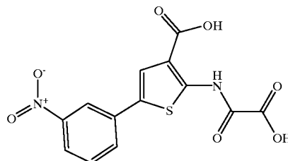
5-(3-Nitro-phenyl)-2-(oxalyl-amino)-thiophene-3-carboxylic acid
