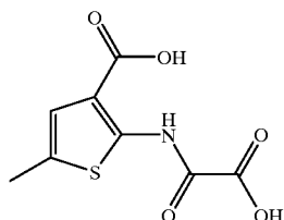
5-Methyl-2-(oxalyl-amino)-thiophene-3-carboxylic acid
