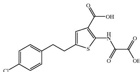
5-(2-(4-Chloro-phenyl)-ethyl)-2-(oxalyl-amino)-thiophene-3-carboxylic acid, mono sodium salt
