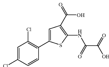
5-(2,4-Dichloro-phenyl)-2-(oxalyl-amino)-thiophene-3-carboxylic acid
