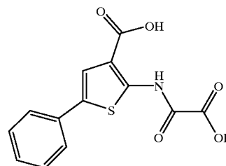
2-(Oxalyl-amino)-5-phenyl-thiophene-3-carboxylic acid
