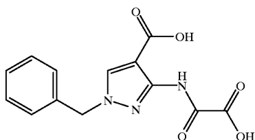
1-Benzyl-3-(oxalyl-amino)-1H-pyrazole-4-carboxylic acid
