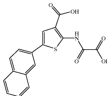
5-(Naphthalen-2-yl)-2-(oxalyl-amino)-thiophene-3-carboxylic acid
