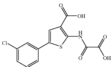
5-(3-Chloro-phenyl)-2-(oxalyl-amino)-thiophene-3-carboxylic acid
