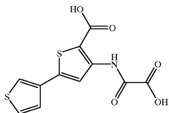
4-(Oxalyl-amino)-[2,3]-bithiophenyl-5-carboxylic acid
