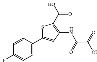
5-(4-Fluoro-phenyl)-3-(oxalyl-amino)-thiophene-2-carboxylic acid
