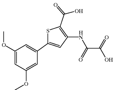
5-(3,5-Dimethoxy-phenyl)-3-(oxalyl-amino)-thiophene-2-carboxylic acid
