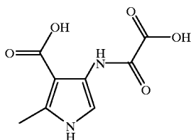
2-Methyl-4-(oxalyl-amino)-1H-pyrrole-3-carboxylic acid
