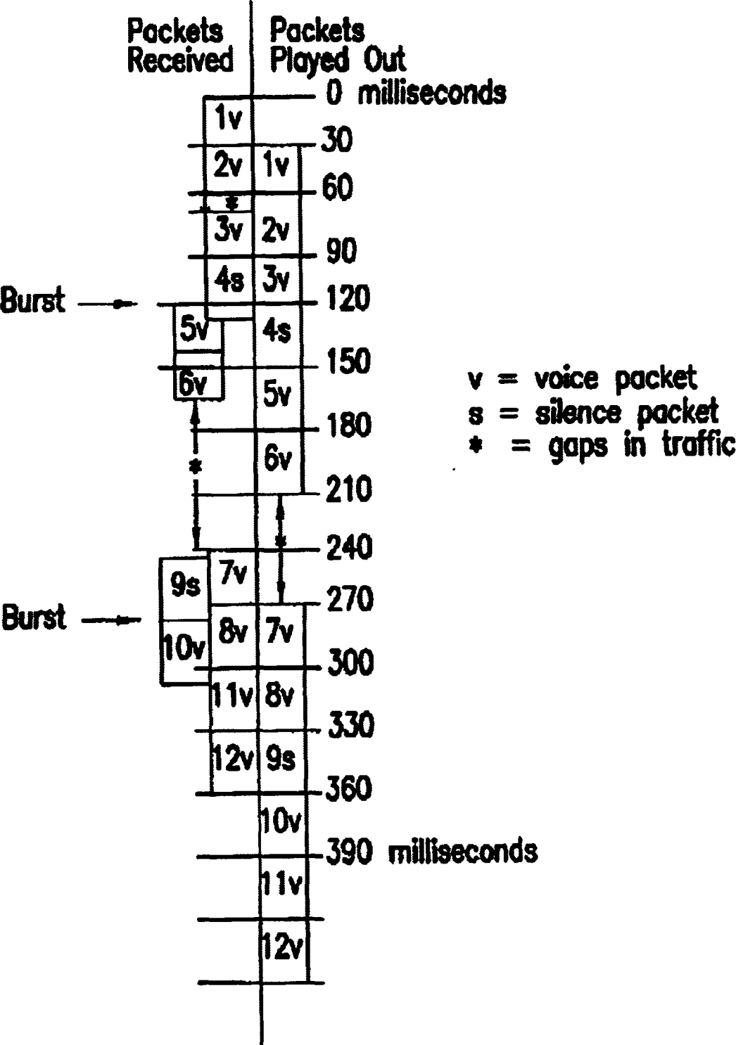
Static Buffering of Jitter
