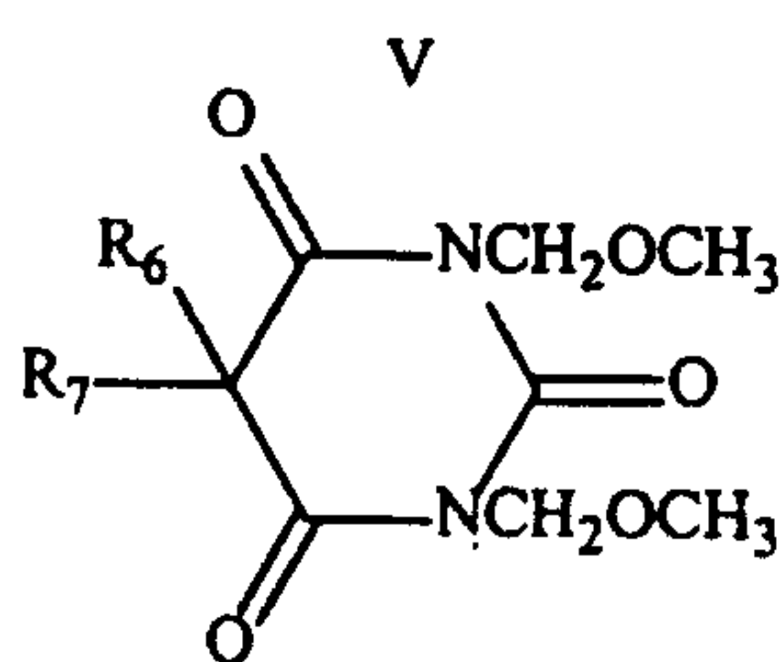
N,N'-bismethoxymethyl-5,5-diphenylbarbituric acid
