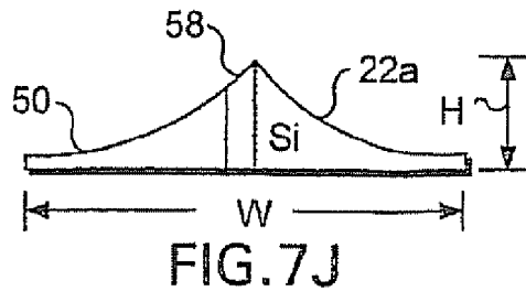
FINISHED MICRO-NEEDLE
