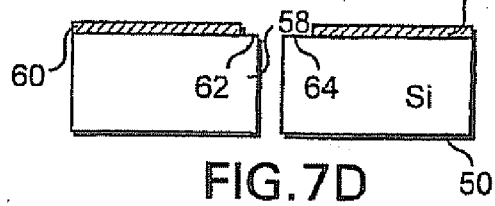
STEP 6. REMOVE NITRIDE PATTERN MASK
