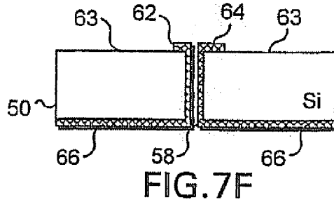
STEP 6. REMOVE NITRIDE PATTERN MASK
