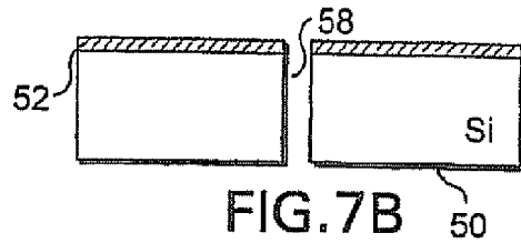
STEP 4. FORM NITRIDE PATTERN MASK
