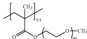
Compound for undercoat layer (2) Mw 100,000
