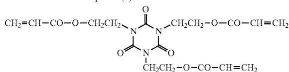
Polymerizable compound (1)
