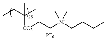
Binder polymer (2)
