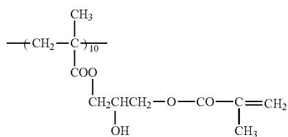
Binder polymer (2)
