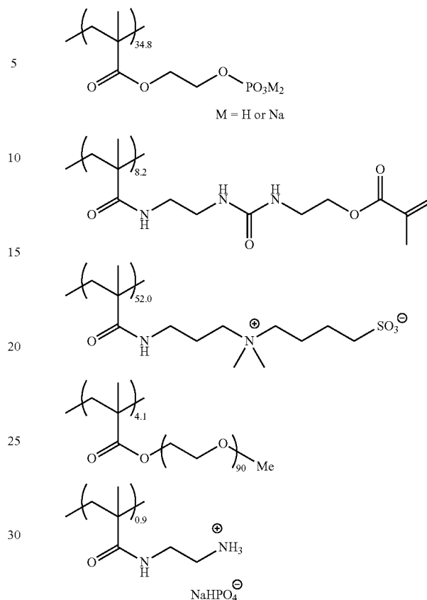
Compound for undercoat layer (UC-2)
