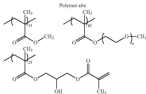
Binder polymer (2) n = 2
