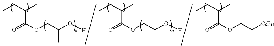
Fluorine-based surfactant
