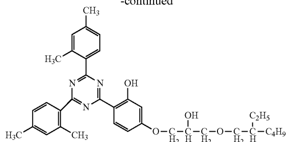
Ultraviolet absorbent (1)
