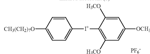
Polymerization initiator (1)
