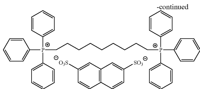
Additive 1
