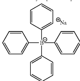
Borate compound (1)
