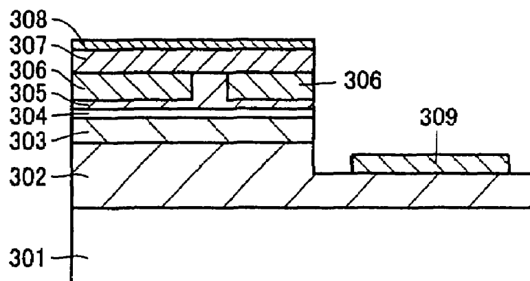
FIG.69 PRIOR ART
