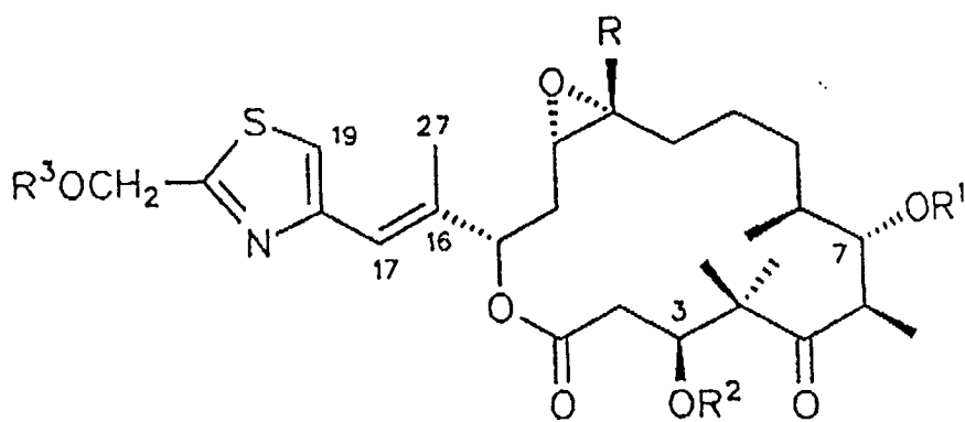
3a R^1, R^2 = H, R^3 = \text{Acetyl}, R = H
