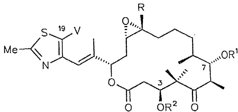
4a R^1, R^2 = H, V = Br, R = H
