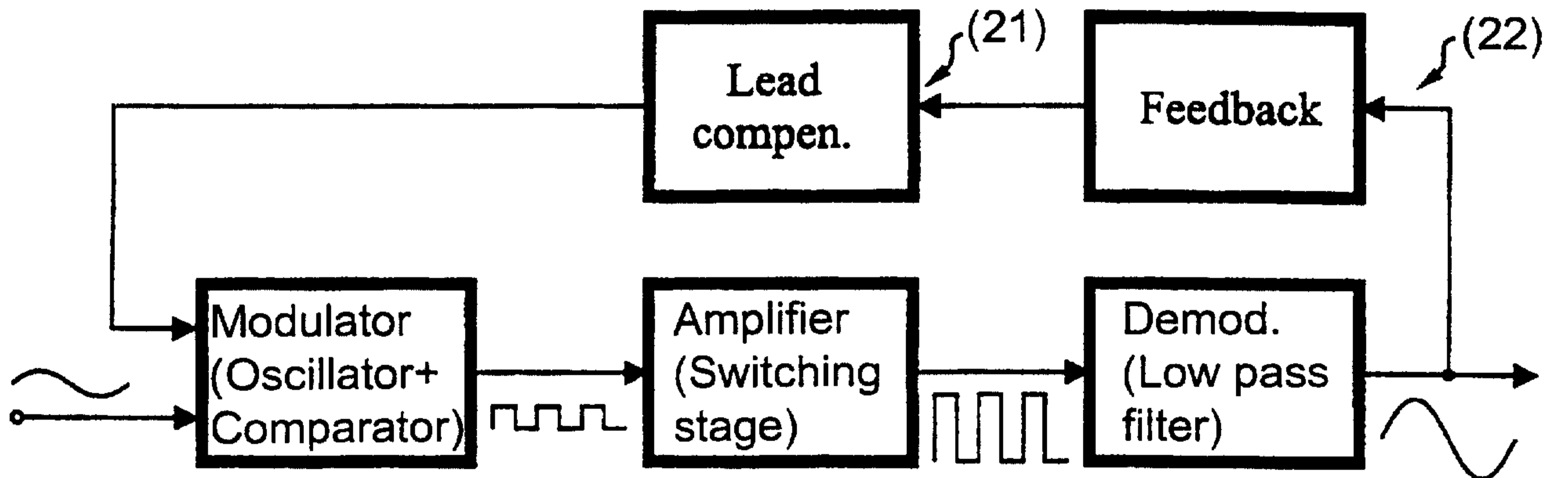
Fig. 2 (Prior art)
