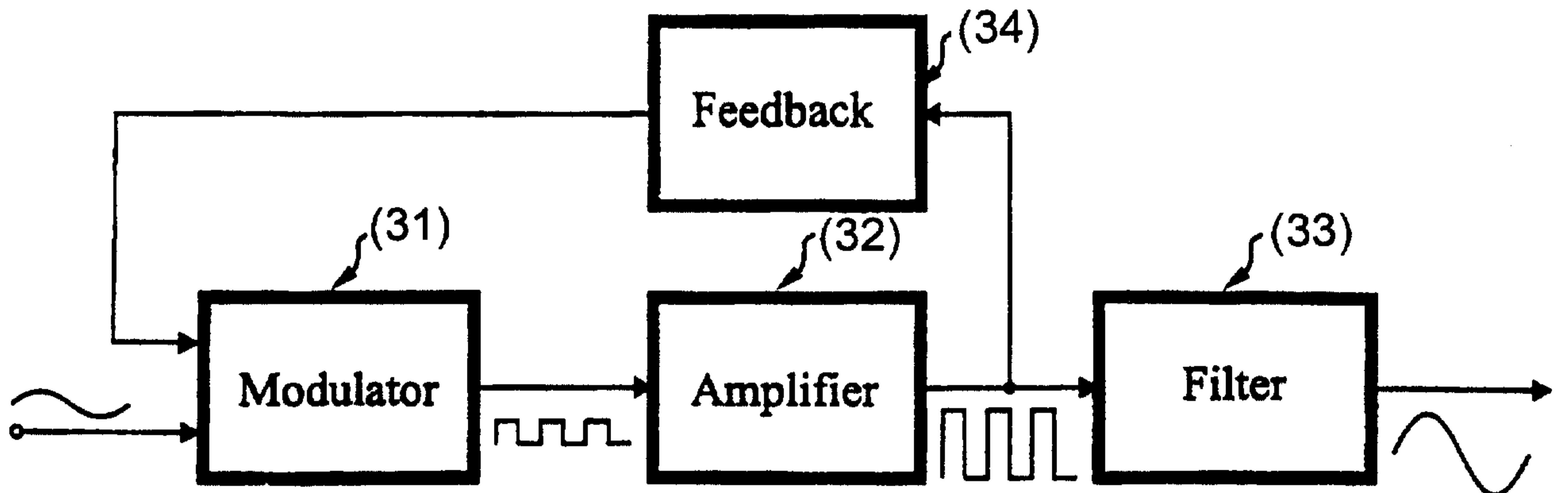
Fig. 3 (Prior art)
