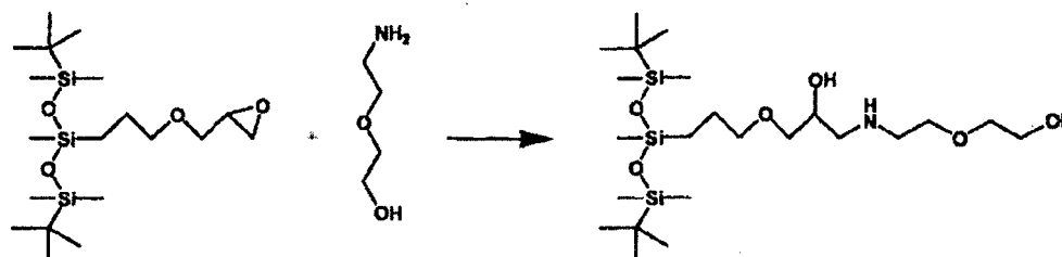
Figure 5. Reaction Sequence for Preparation of Trisiloxane Surfactant 5.
