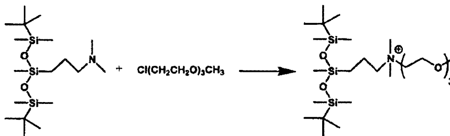
Figure 11. Reaction Sequence for Preparation of Trisiloxane Surfactant 11.
