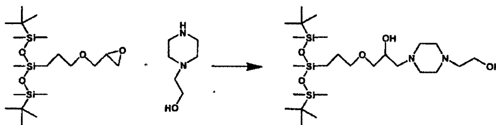
Figure 4. Reaction Sequence for Preparation of Trisiloxane Surfactant 4.
