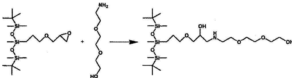
Figure 6. Reaction Sequence for Preparation of Trisiloxane Surfactant 6.
