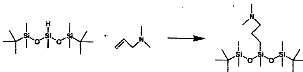
Figure 7. Reaction Sequence for Preparation of Trisiloxane Amine Intermediate 7.
