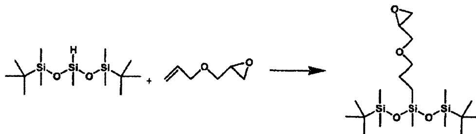
Figure 3. Reaction Sequence for Preparation of Epoxide Intermediate 3.
