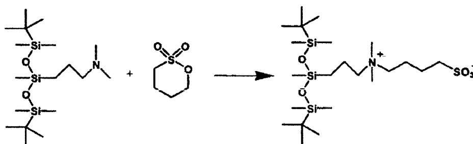
Figure 9. Reaction Sequence for Preparation of Trisiloxane Surfactant 9.
