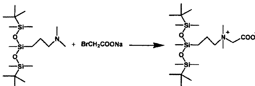
Figure 10. Reaction Sequence for Preparation of Trisiloxane Surfactant 10.
