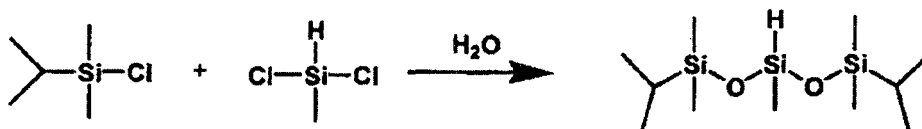
Figure 2. Reaction Sequence for Preparation of Hydride Intermediate 2.
