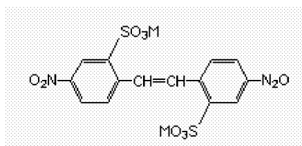
General Formula (III)
