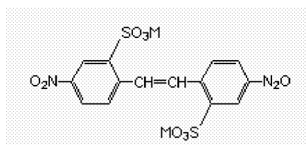
General Formula (III)
