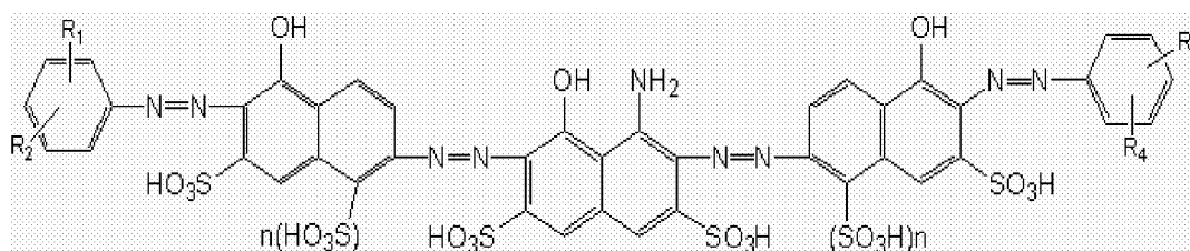
General Formula (I)
