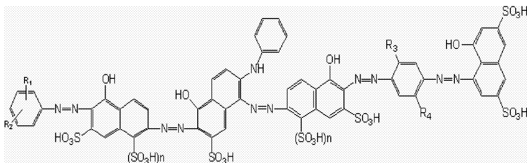
General Formula (II)
