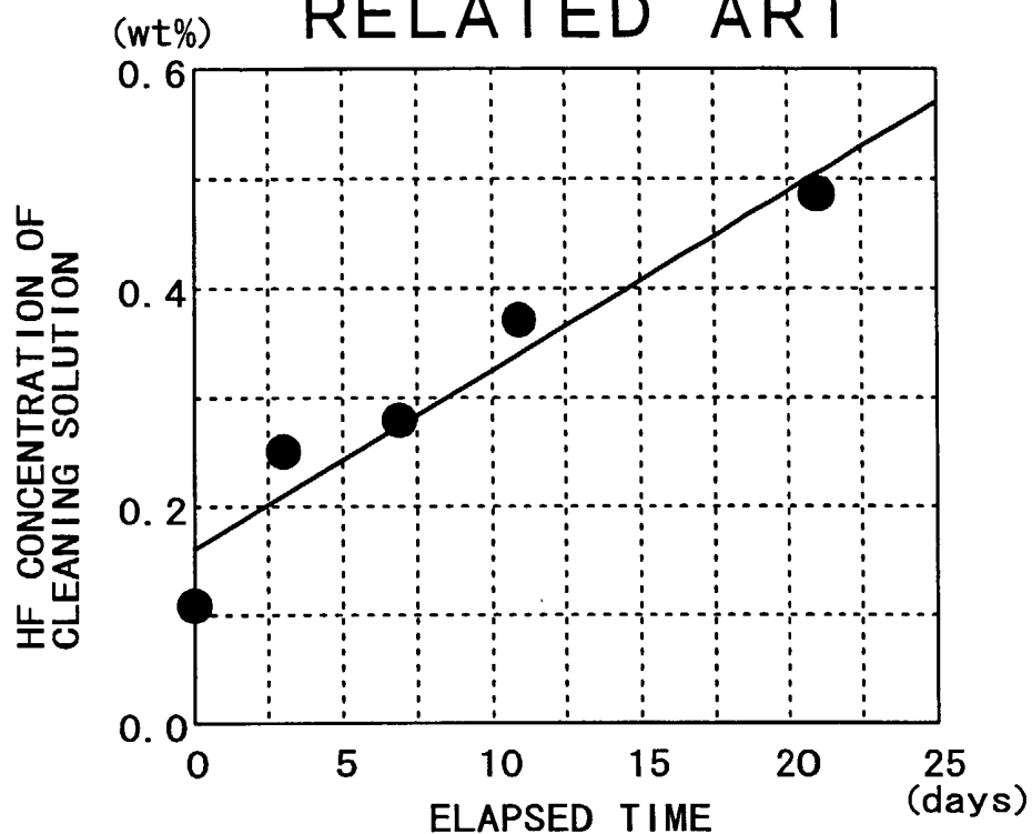
FIG. 7 RELATED ART
