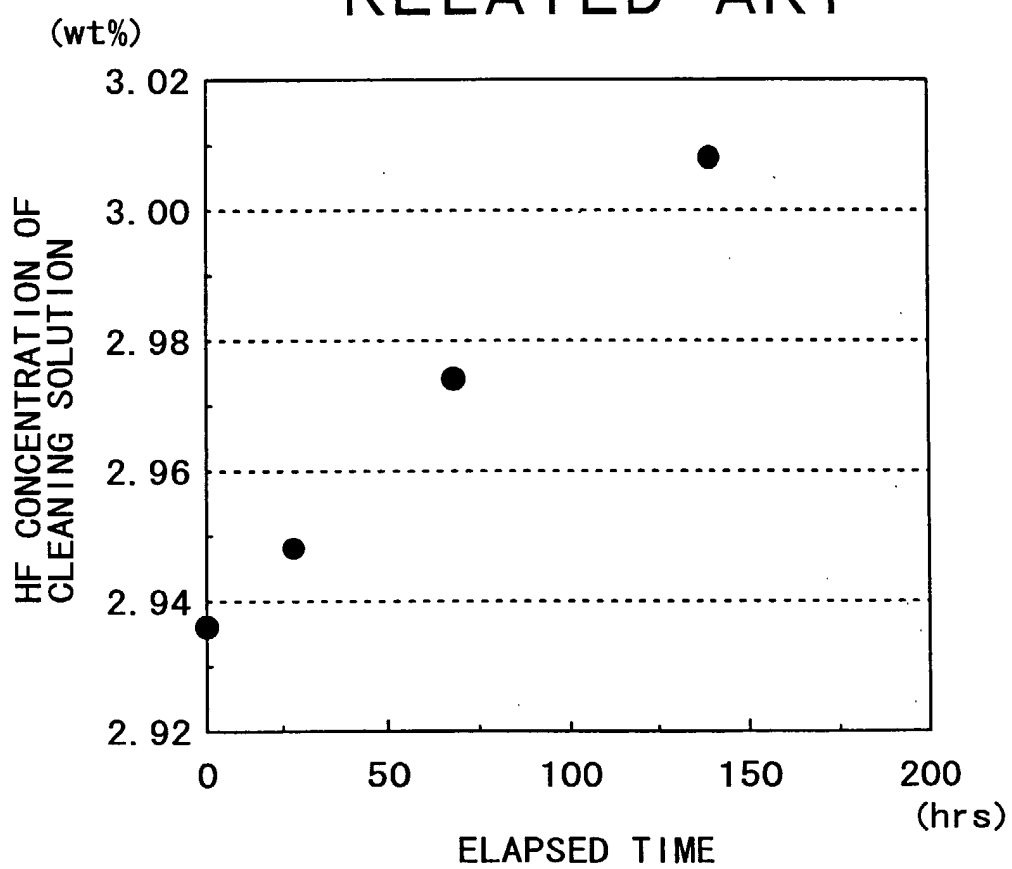
FIG. 1 RELATED ART
