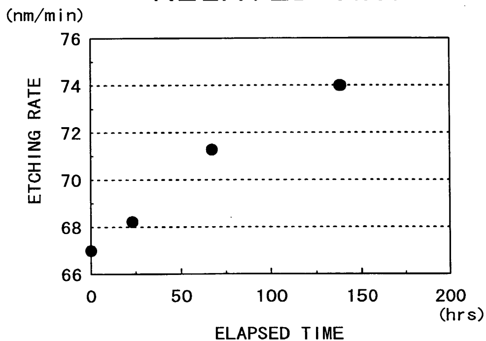
FIG. 2 RELATED ART
