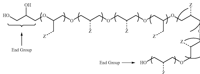
UV-ABSORBING POLYGLYCEROL
