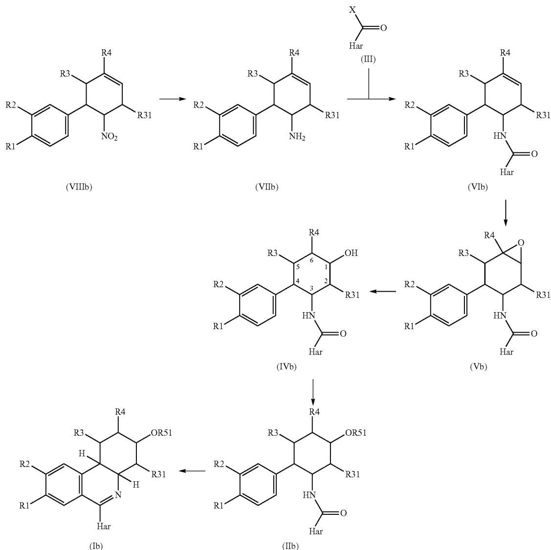
Reaction scheme 3:
