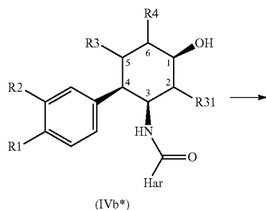
Reaction scheme 4:
