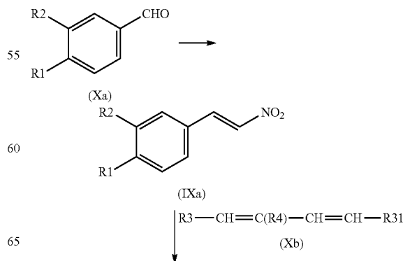
Reaction scheme 5:
