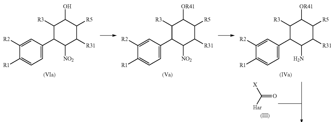
Reaction scheme 1:
