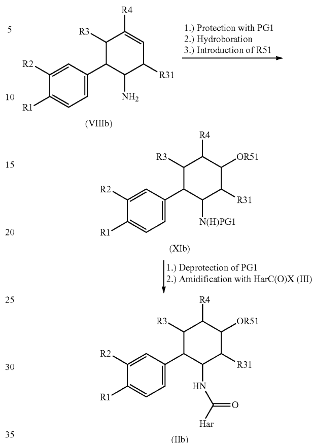
Reaction scheme 6:
