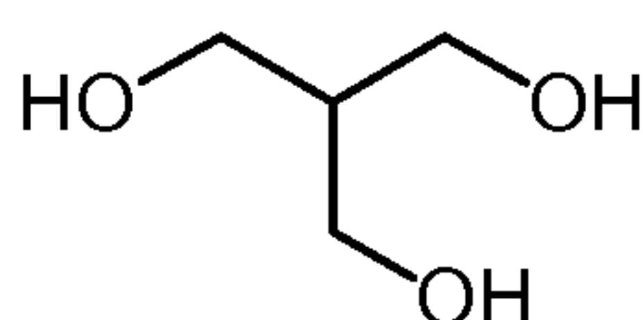
2-(hydroxymethyl)-1,3-propanediol
