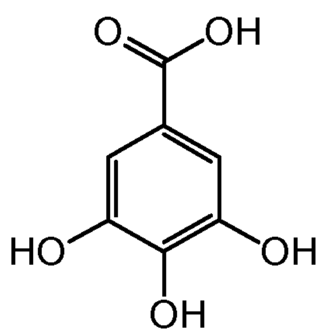
Gallic acid
