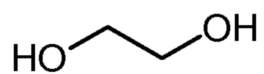
Ethylene glycol
