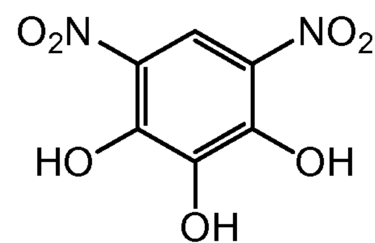
4,6-Nitropyrogallol
