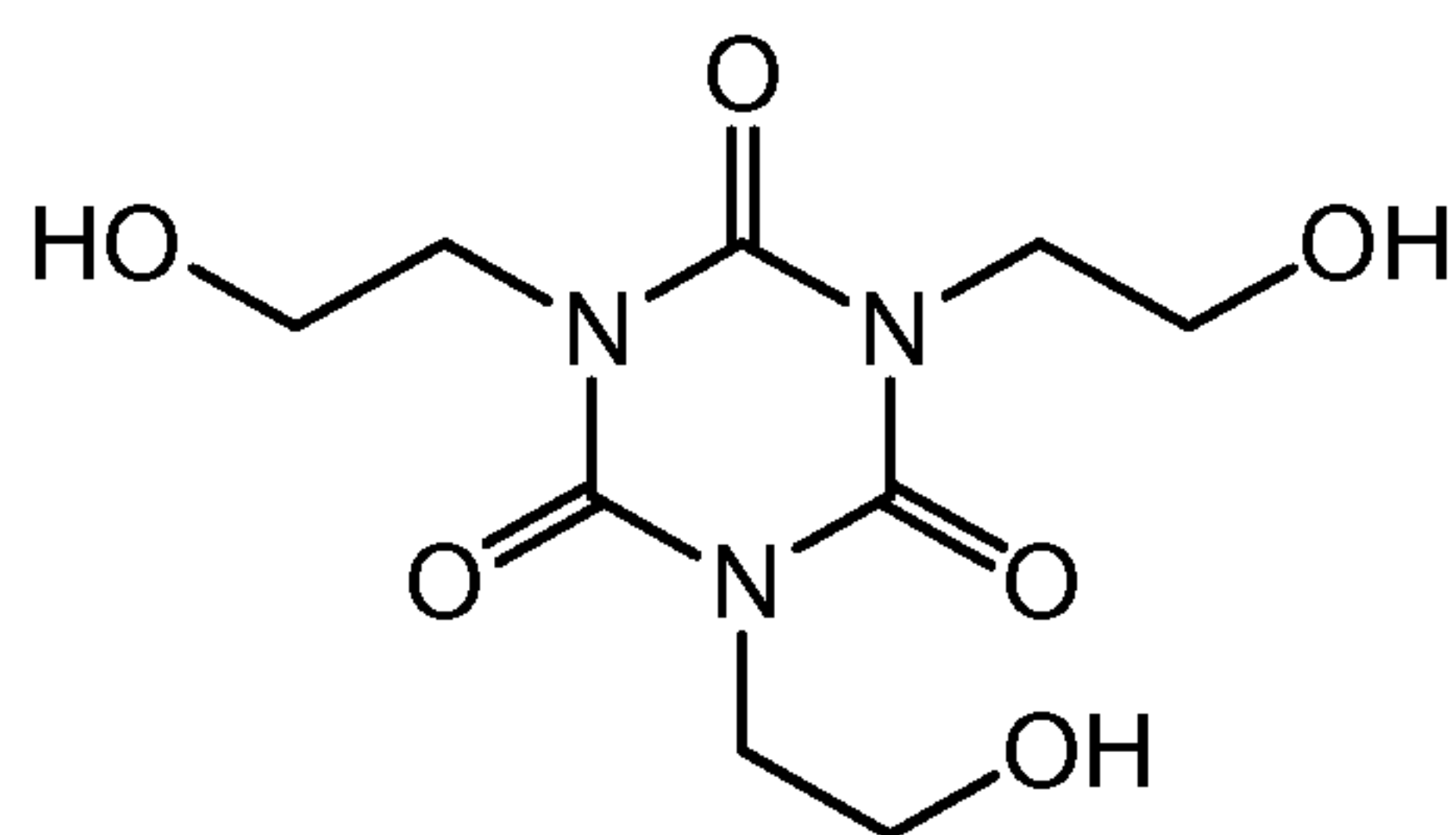
1,3,5-Tris(2-hydroxyethyl)-Cyanuric acid
