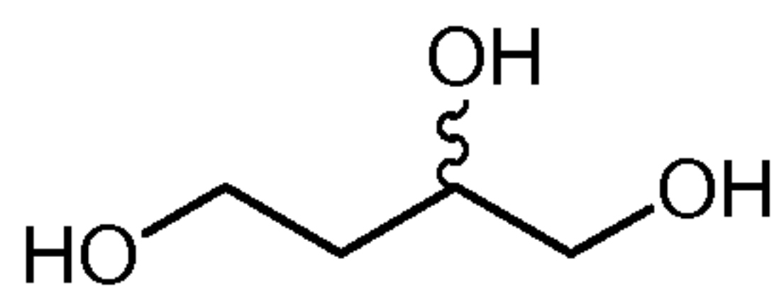
1,2,4-Butanetriol
