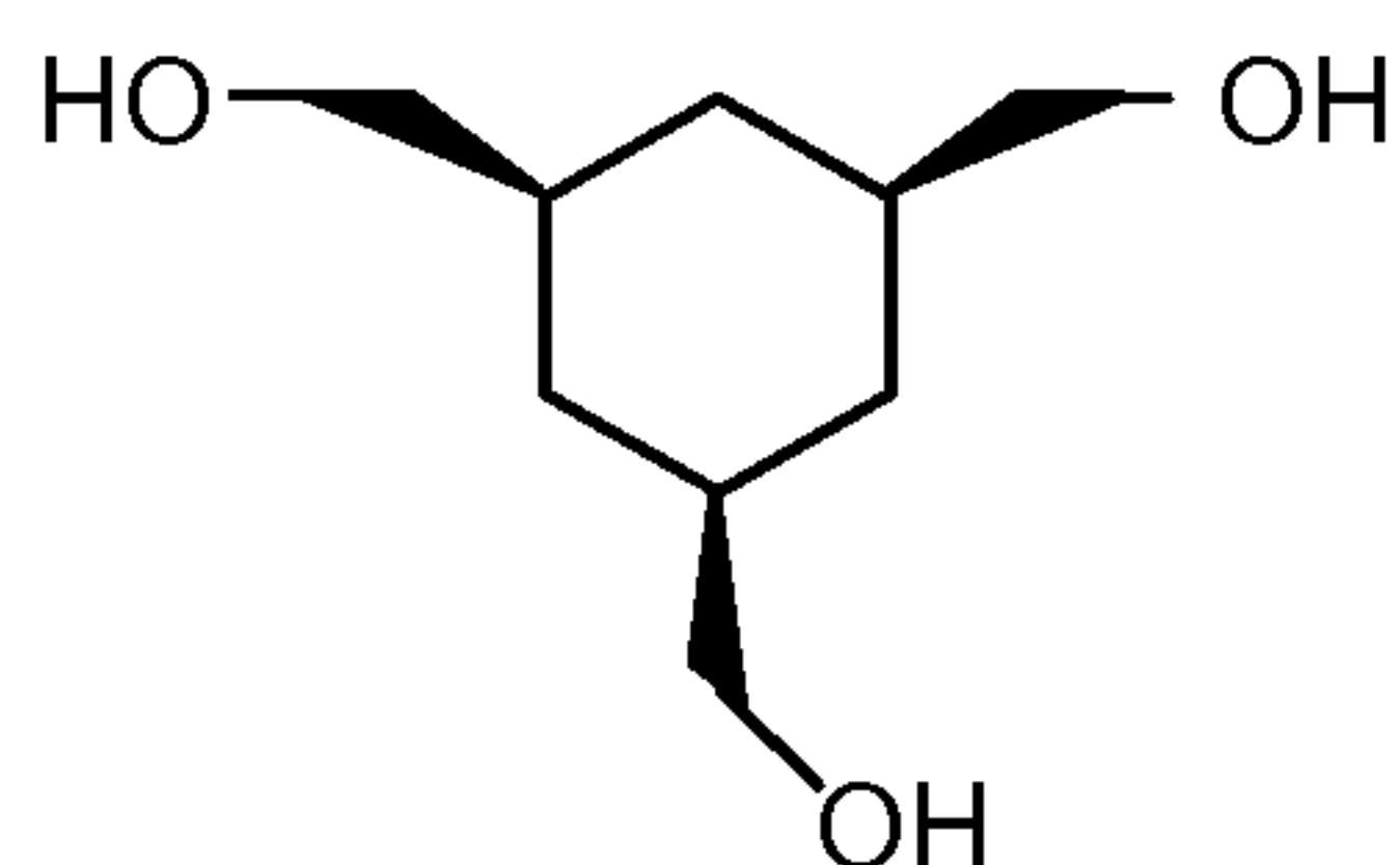
cis-1,3,5-Tri(hydroxymethyl)cyclohexane
