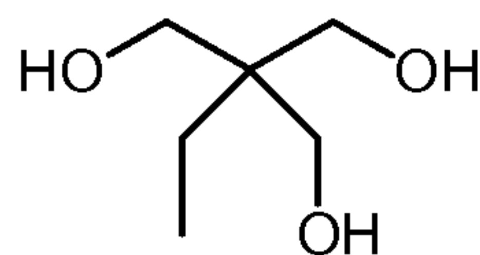
1,1,1-Tris(hydroxymethyl)propane
