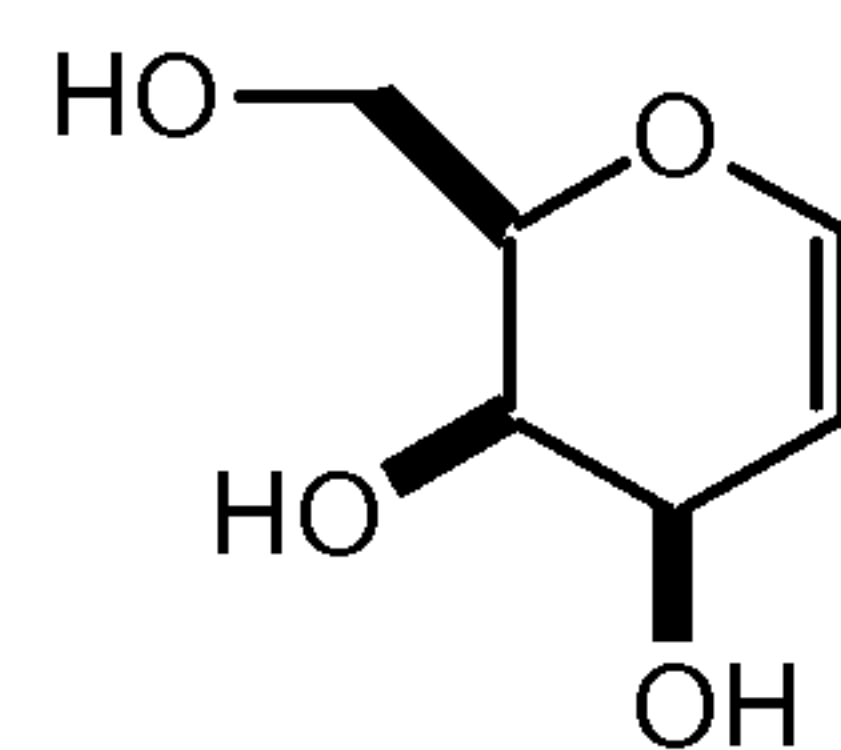
D-Galactal
