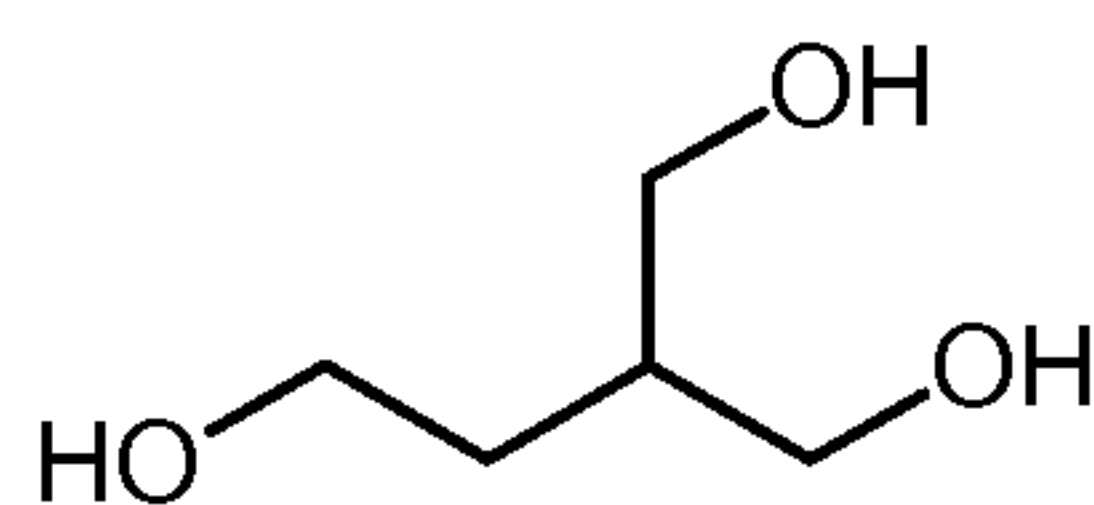
2-(hydroxymethyl)1,4-butanediol
