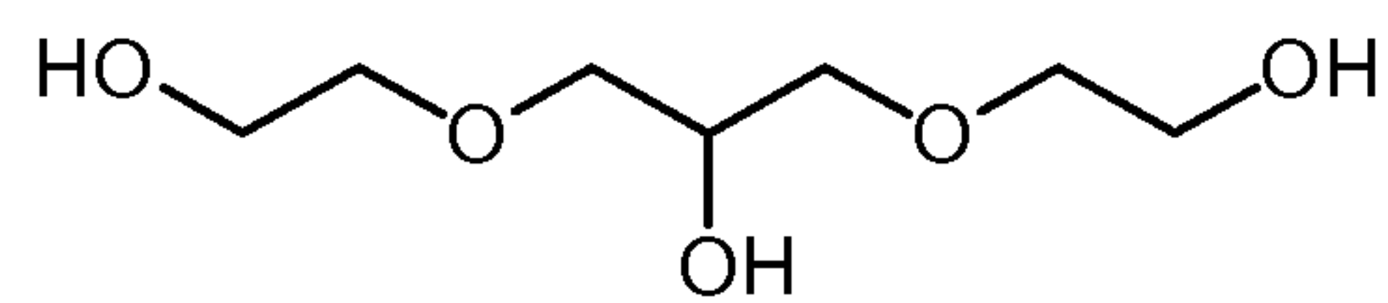
1,3-Di(hydroxyethoxy)-2-hydroxyl-propane
