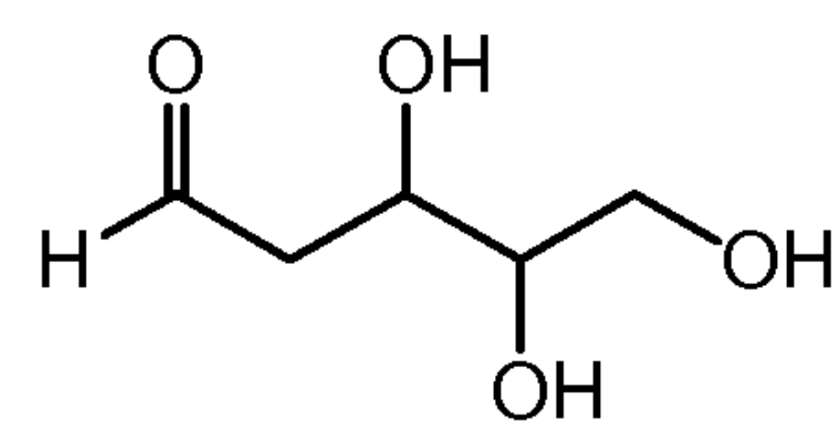
2-Deoxy-D-ribose
