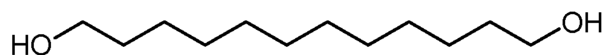
1,12-Dodecanediol
