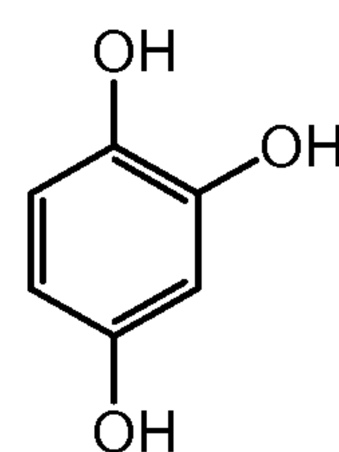
1,2,4,-Trihydroxyl-benzene
