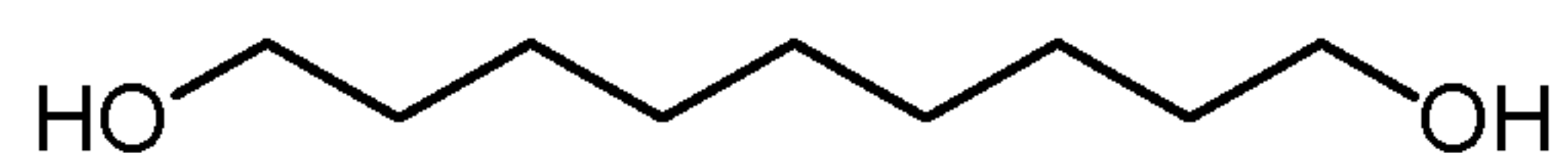
1,9-Nonanediol
