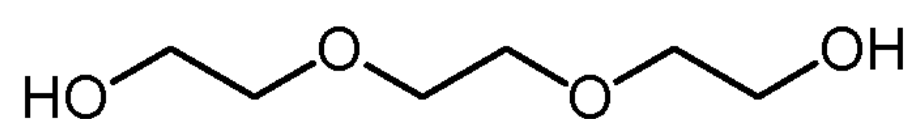
Triethylene glycol
