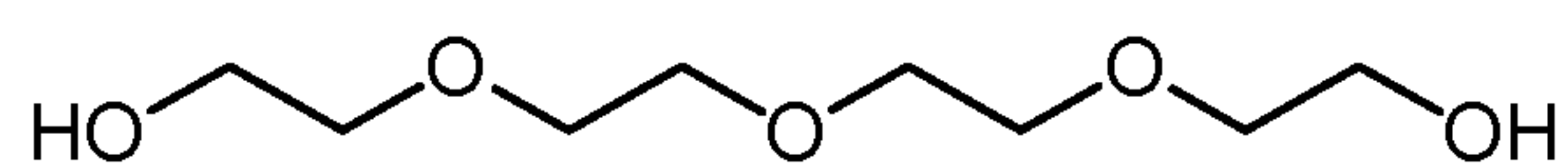
Tetraethylene glycol
