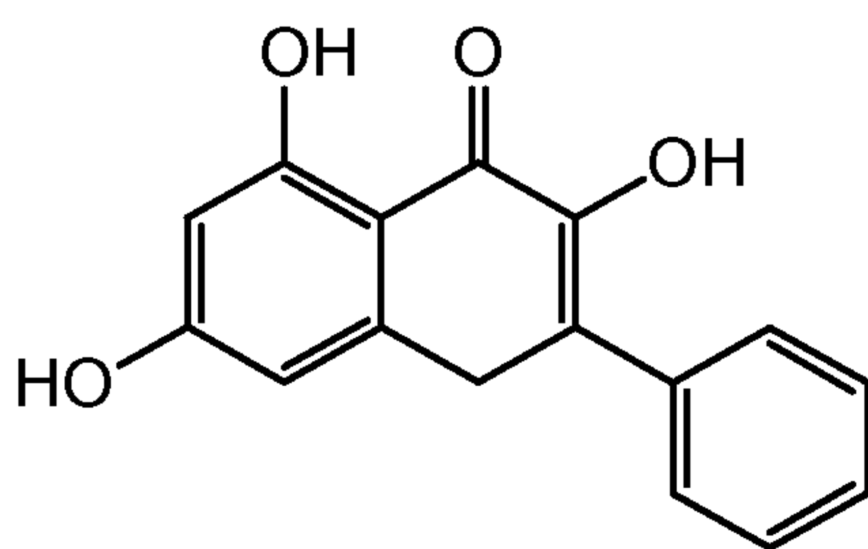
3,5,7-Trihydroxyflavone
