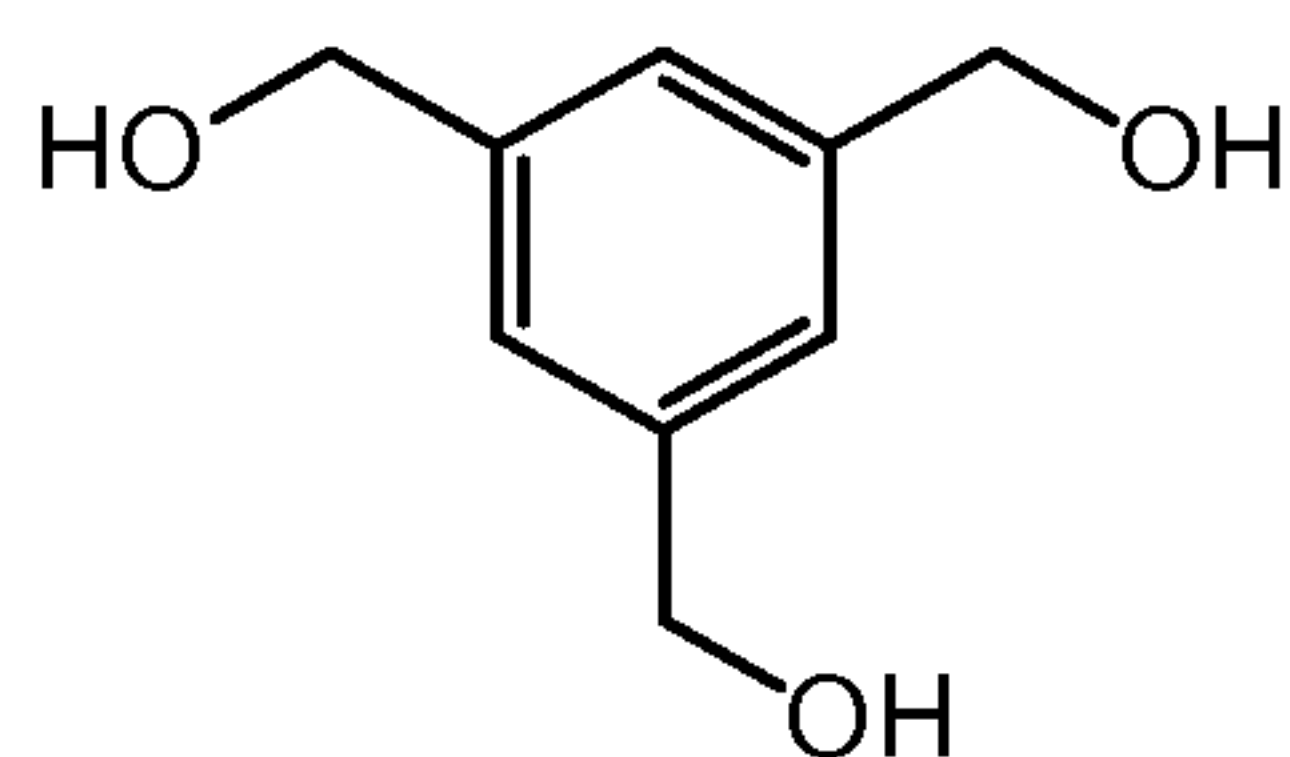
1,3,5,-Tri(hydroxymethyl)benzene
