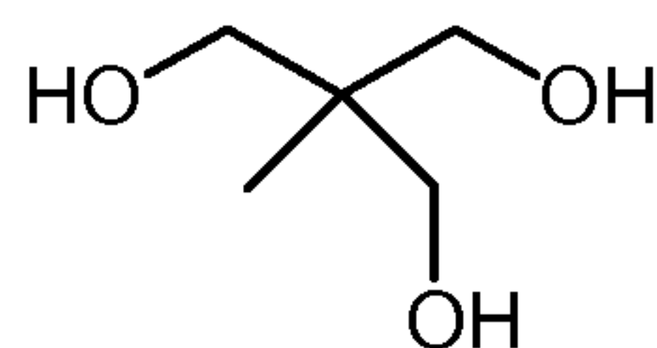
1,1,1-Tris(hydroxymethyl)ethane
