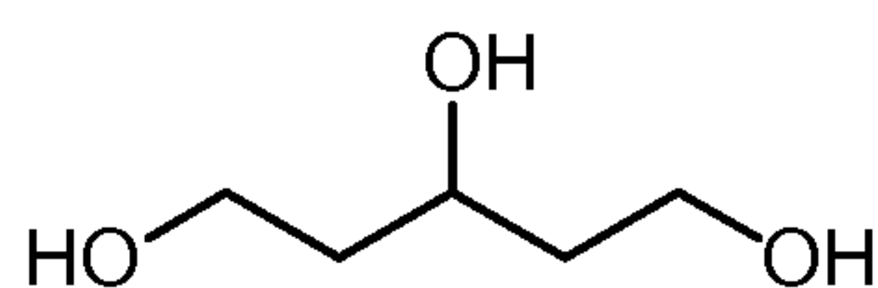
1,3,5-Pentanetriol
