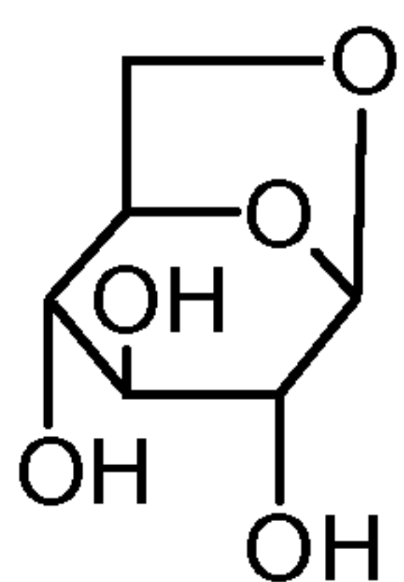
1,6-anhydro- \beta -D-Glucose
