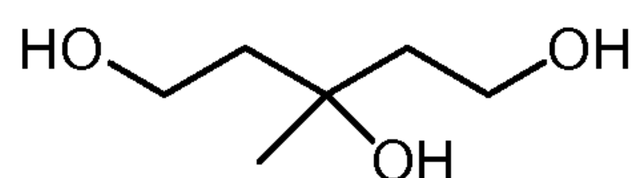
3-Methyl-1,3,5-pentanetriol
