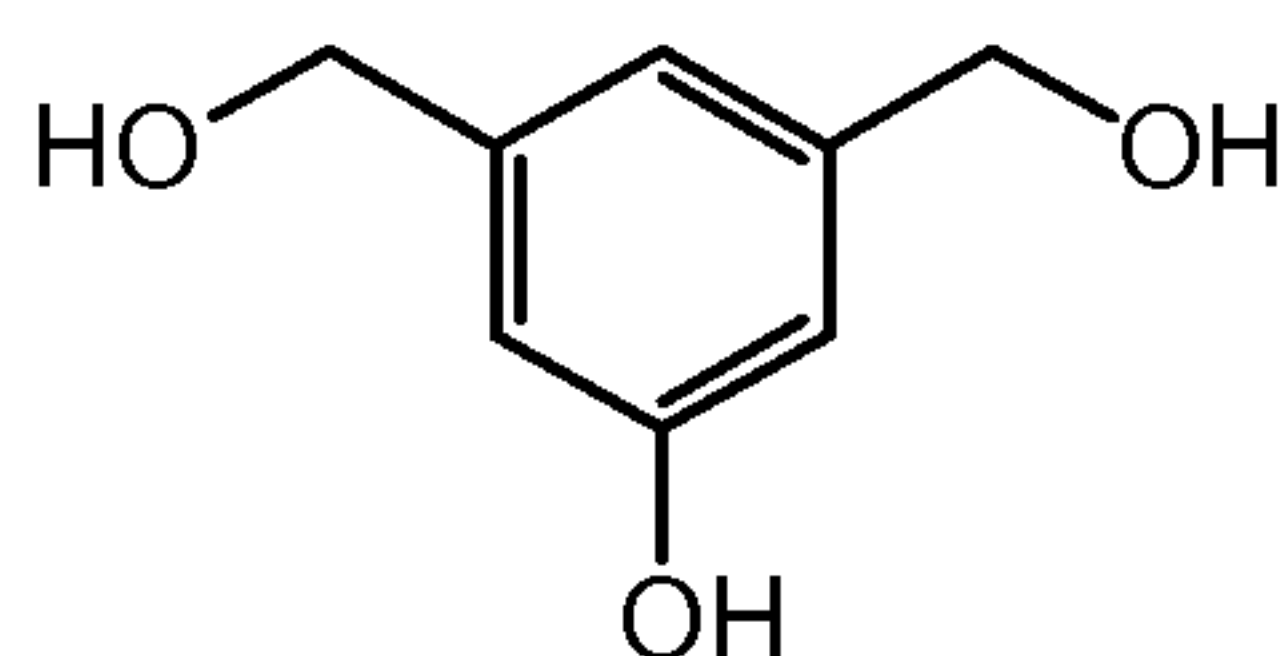
3,5,-Di(hydroxymethyl)phenol
