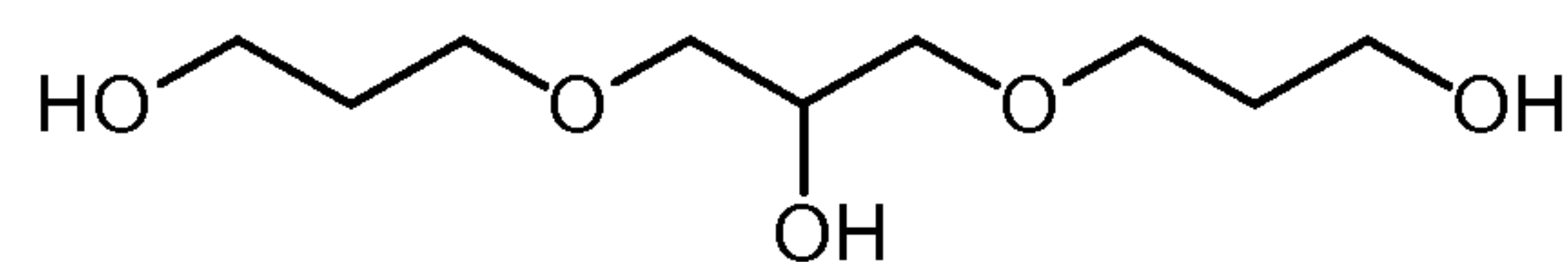
1,3-Di(hydroxypropoxy)-2-hydroxyl-propane
