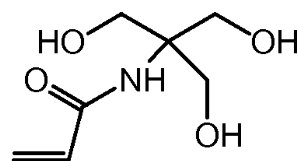
N-[Tris(hydroxymethyl)methyl]acrylamide
