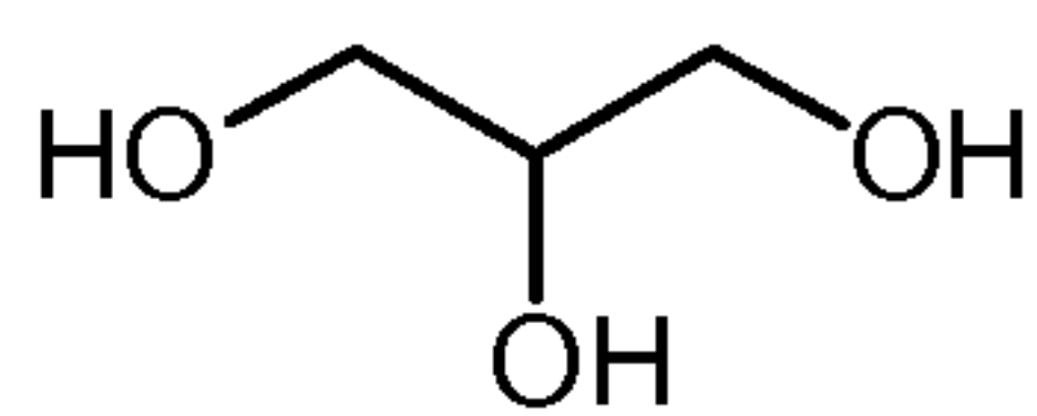
Glycerol (1,2,3-Propanetriol)
