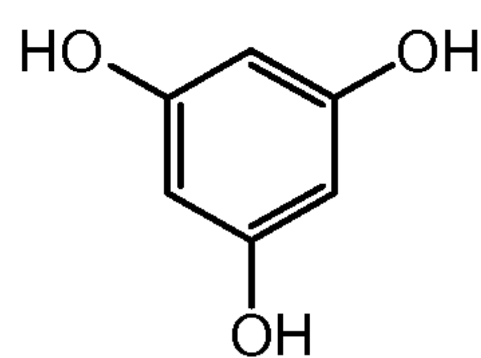
1,3,5,-Trihydroxyl-benzene
