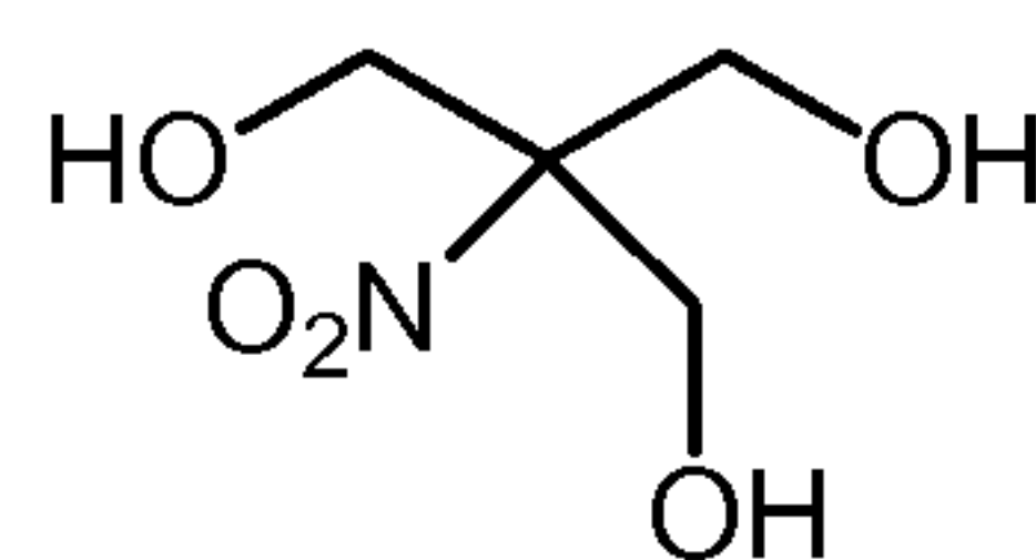
1,1,1-Tris(hydroxymethyl)nitromethane
