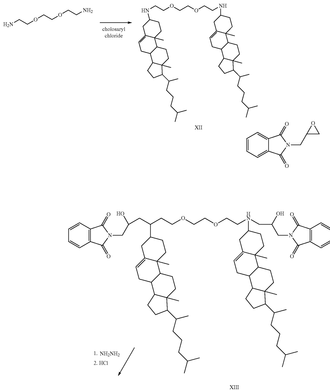
Synthesis of cholesterol analogs (Scheme 3)
