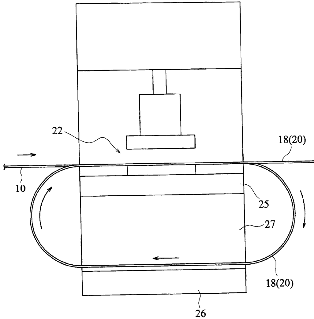
FIG. 3 (PRIOR ART)
