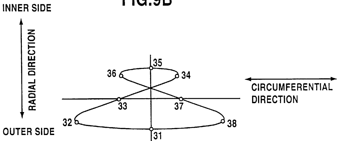
POSITION OF BALLS IN POCKETS OF CAGE AT INCORPORATION ANGLE \alpha (IN A CASE WITH CAGE OFFSET)
