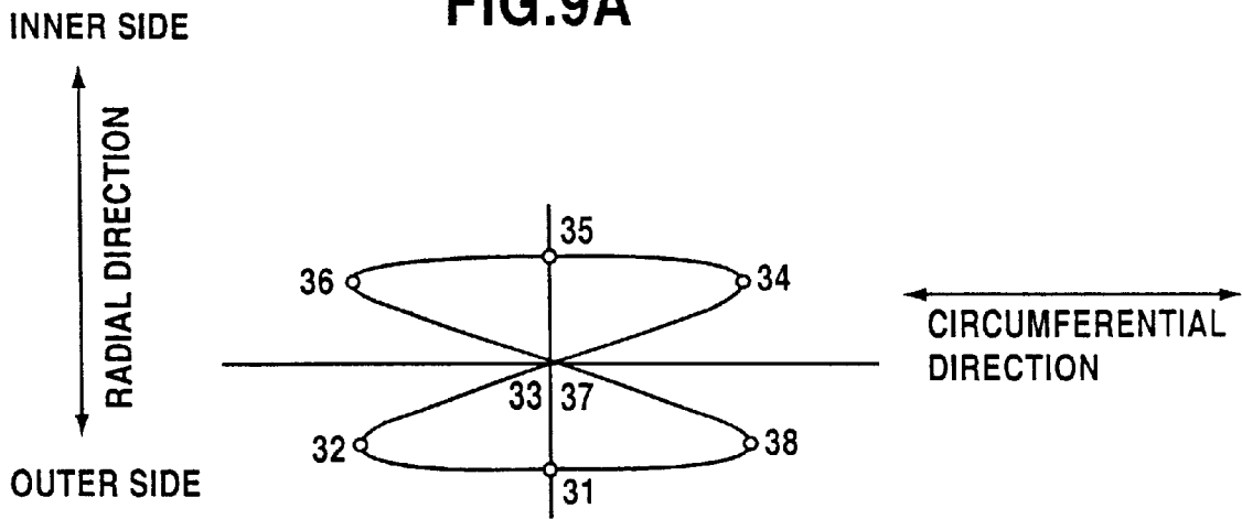
POSITION OF BALLS IN POCKETS OF CAGE AT INCORPORATION ANGLE \alpha (IN A CASE WITHOUT CAGE OFFSET)
