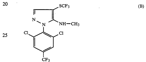
1-(2,6-Dichloro-4-trifluoromethylphenyl)-5-methylamino-4-trifluoromethylthio-pyrazole (both known from EP 201,852)
