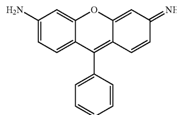
Rosamine
