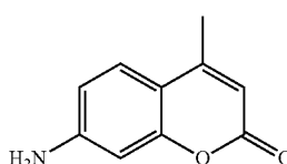
7-Amino-4-methylcoumarin
