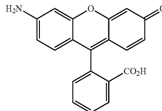
Rhodol
