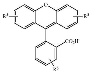
Scheme I
