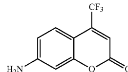
7-Amino-4-trifluoromethylcoumarin
