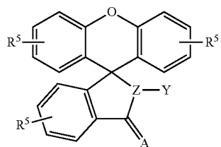
Scheme IV
