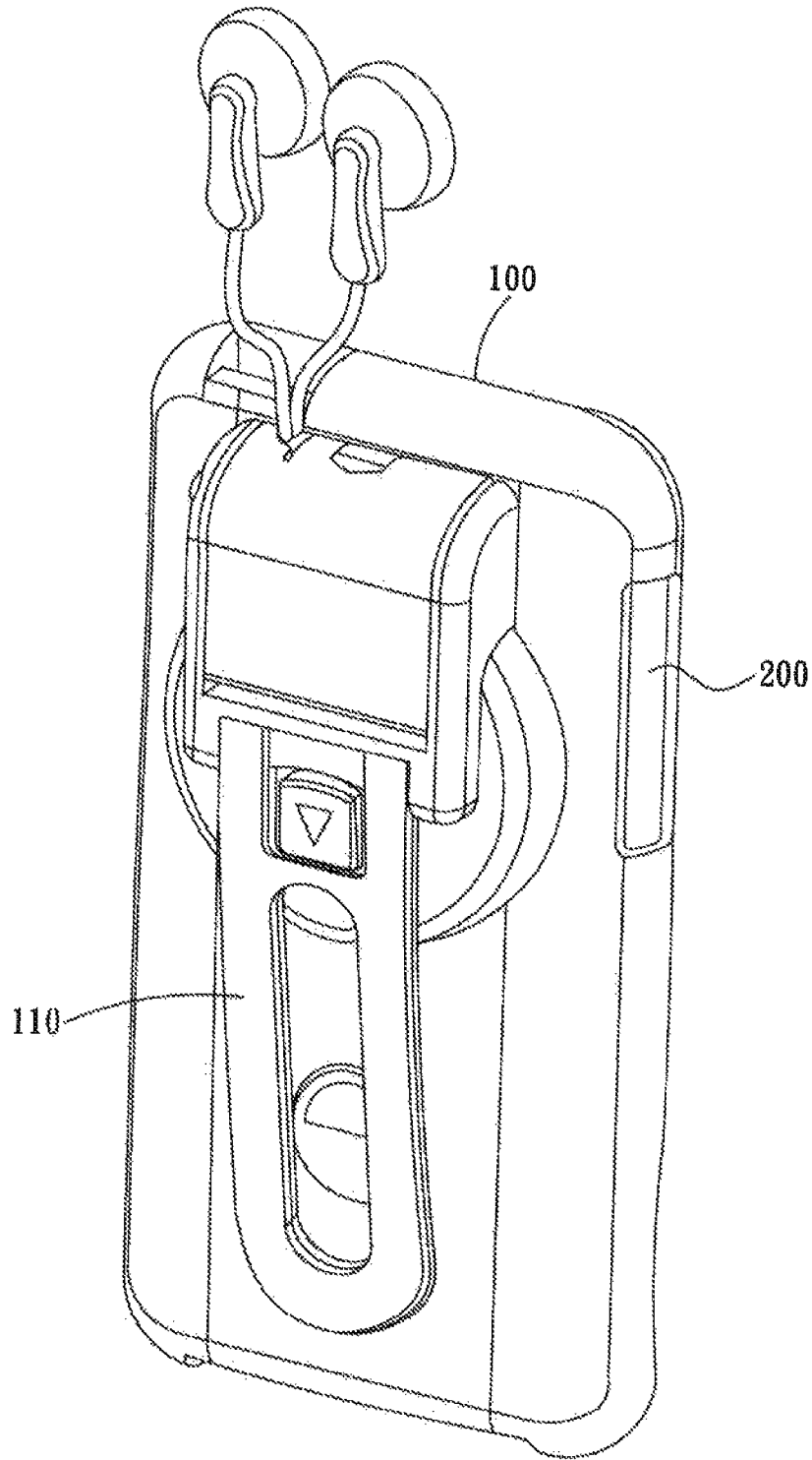
FIG. 1 (Prior art)
