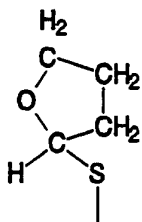
Tetrahydrofuranyl
