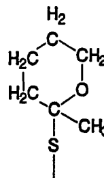
2-methyl tetrahydropyranyl
