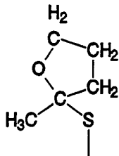
2-methyl tetrahydrofuranyl
