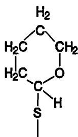
Tetrahydropyranyl
