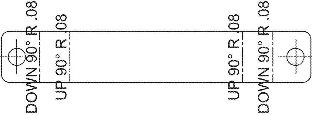
FLAT PATTERN FIG. 9B
