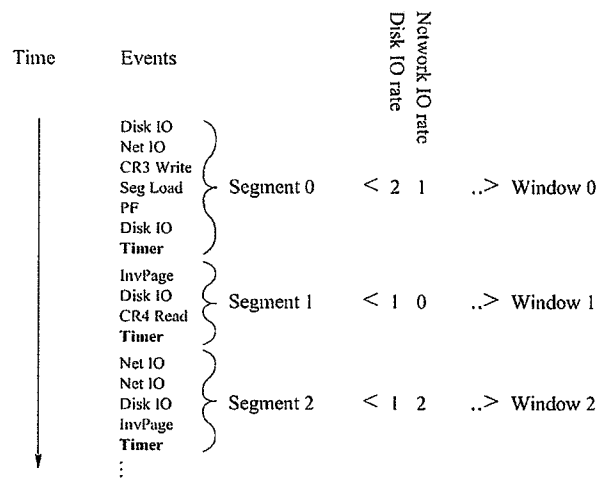
Figure 2: Constructing Features. Events (a) → Basic features (b)
