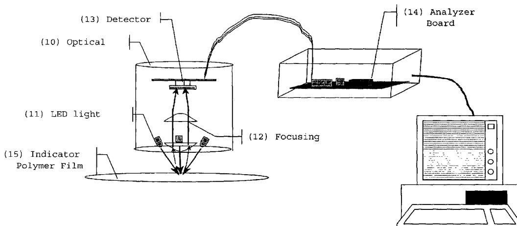
Optical instrumentation used for lifetime measurements
