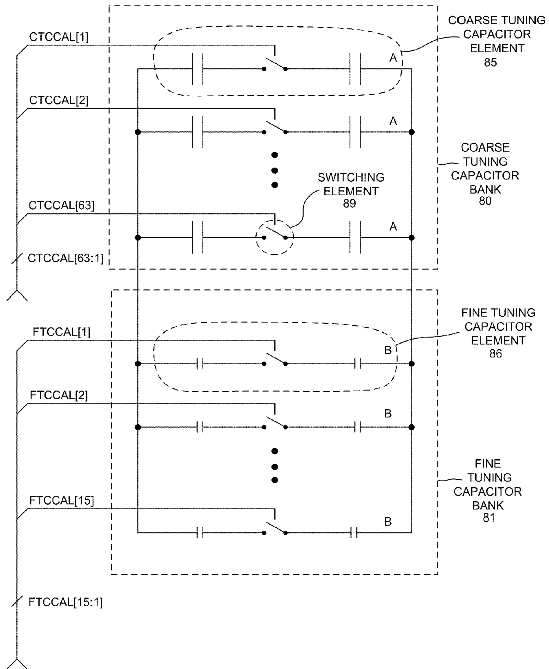
DIGITAL CONTROL OF OVERLAPPING, TWO-SEGMENT CAPACITOR BANK
