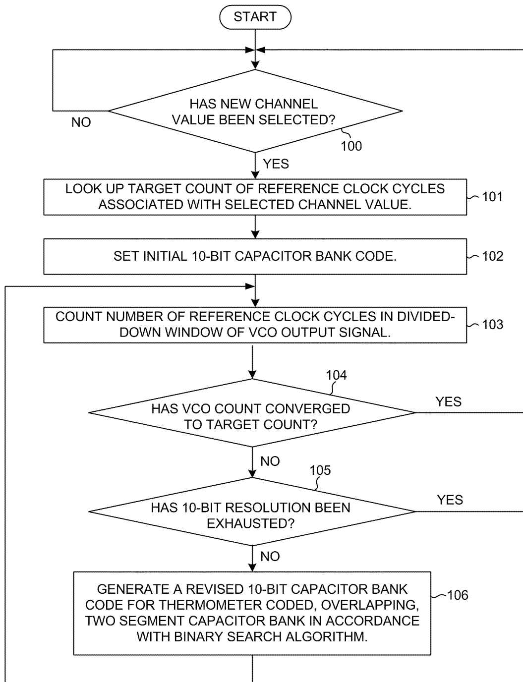
METHOD FOR SELECTING CAPACITOR BANK CODE
