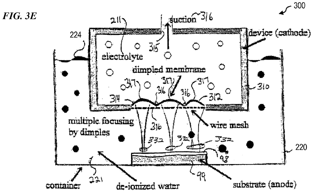
Device for FEFI parallel processing.
