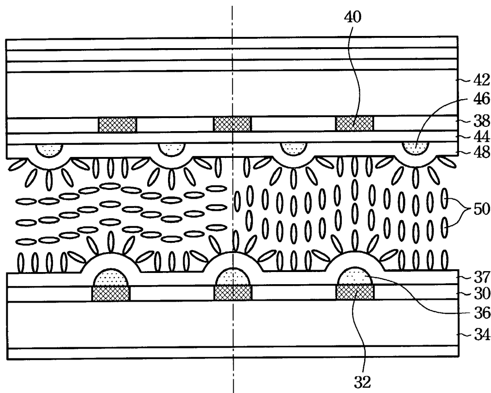
Fig. 3 (Prior Art)
