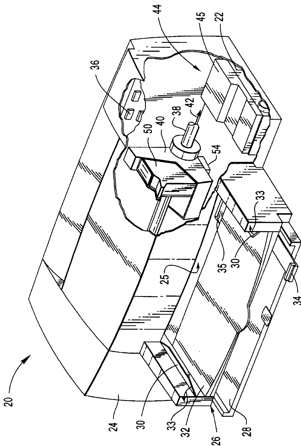
Figure 1 (Prior Art)
