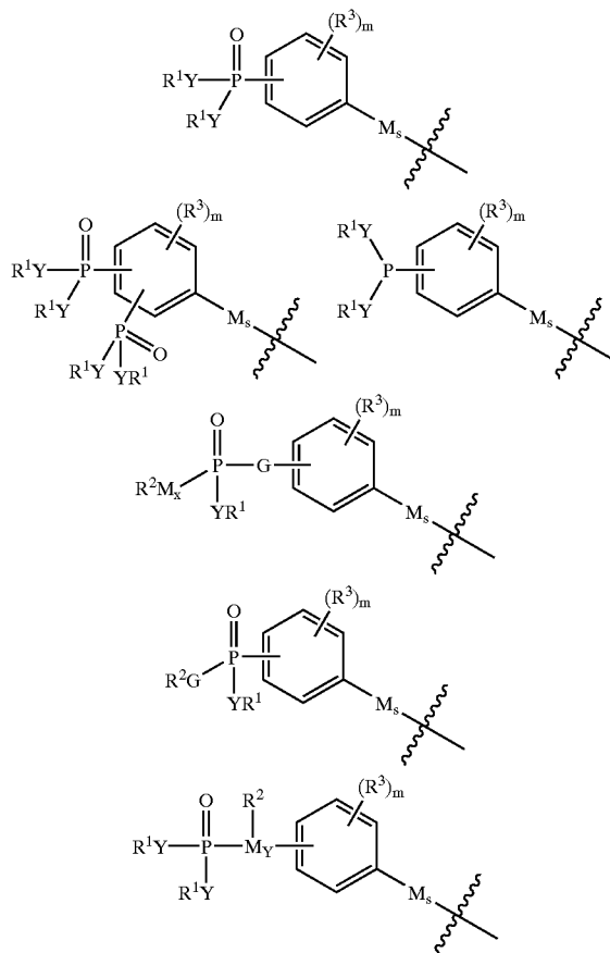
Series IIC
