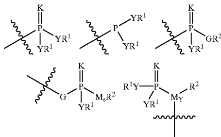
Series I
