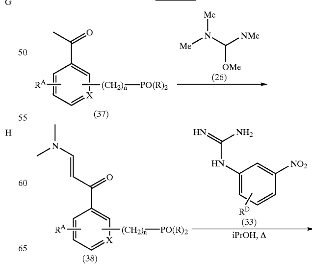
Scheme 15
