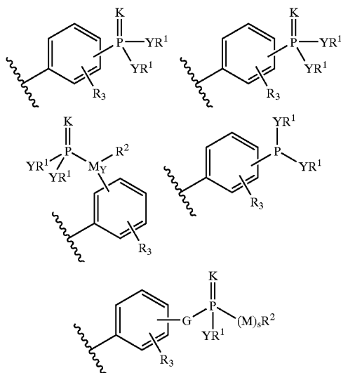
Series IIB
