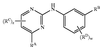
Formula Ia
