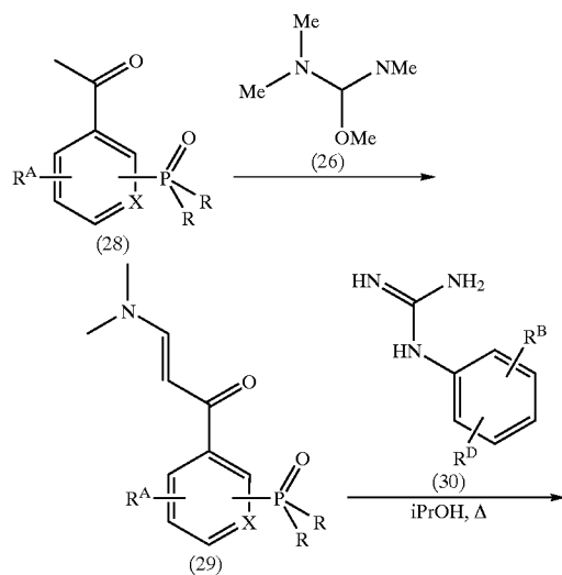
Scheme 11
