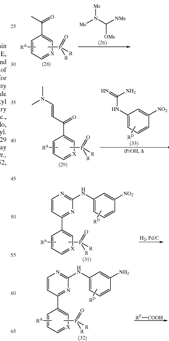
Scheme 12
