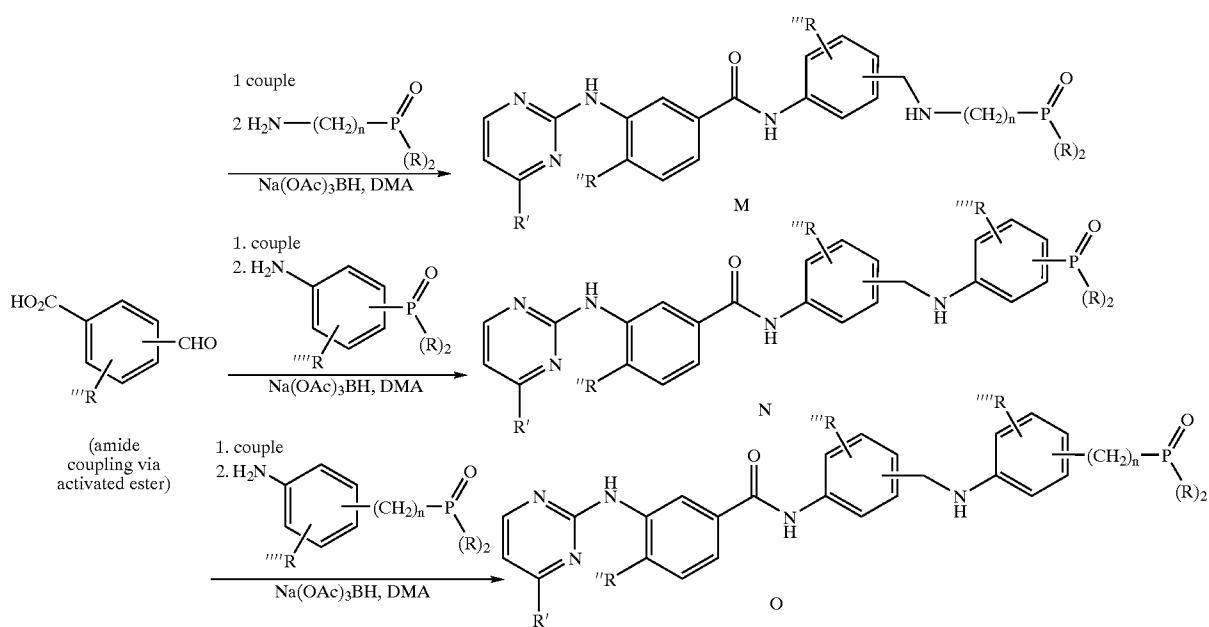
Scheme 31
