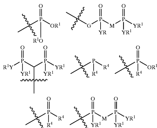
Series Ia
