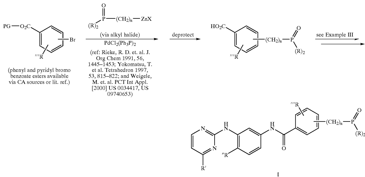
Scheme 30
