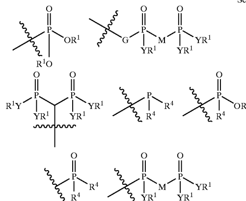
Series Ia
