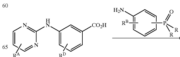
Scheme 20
