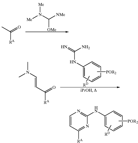
Scheme 26
