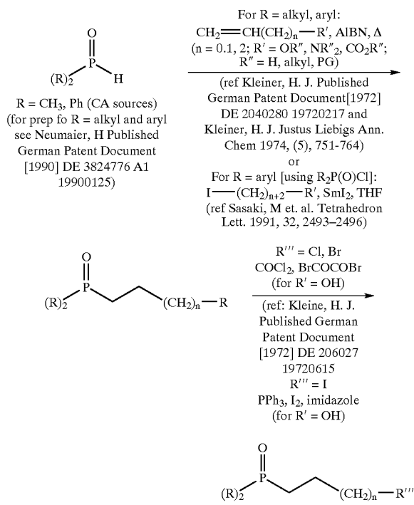
Scheme 8
