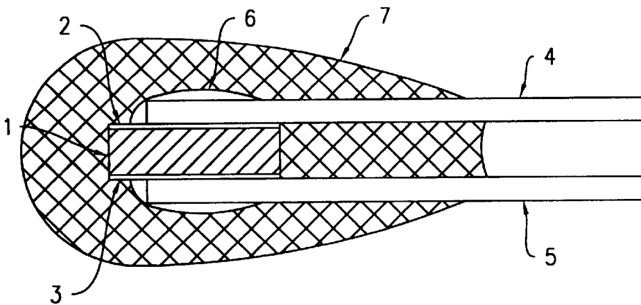
(PRIOR ART) FIG. 2B
