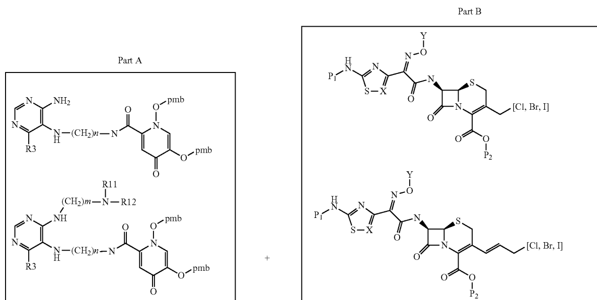
<Reaction Scheme 1>
