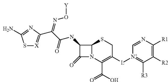
[Chemical Formula 1]
