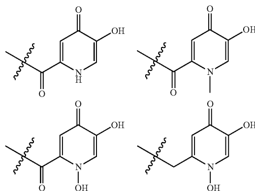
[Chemical Formula 2]
