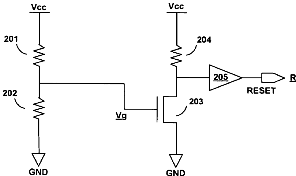
FIGURE 2 (CONVENTIONAL ART)
