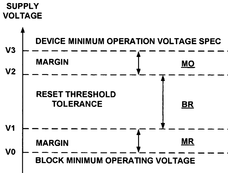
FIGURE 1 (CONVENTIONAL ART)
