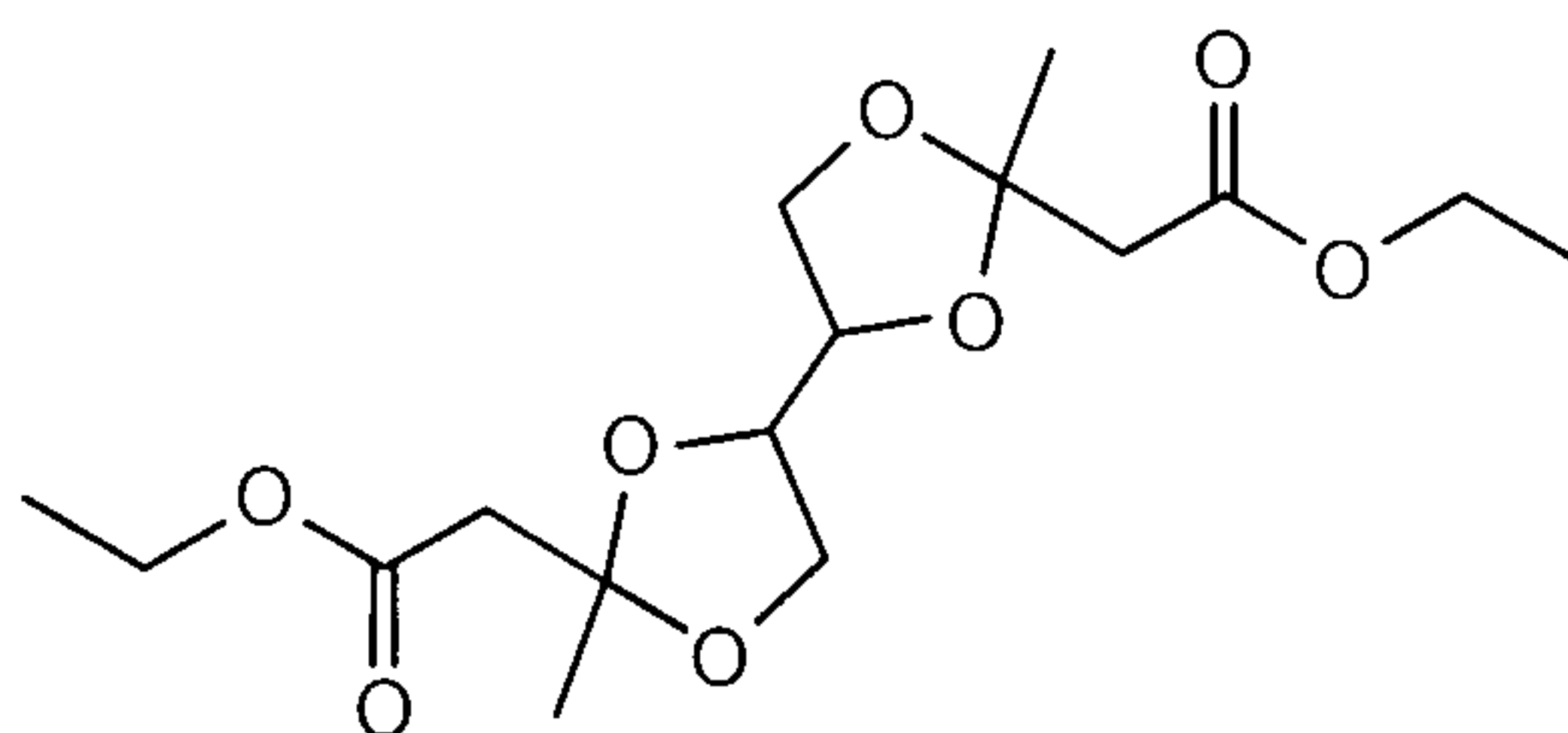
EtBAEK
