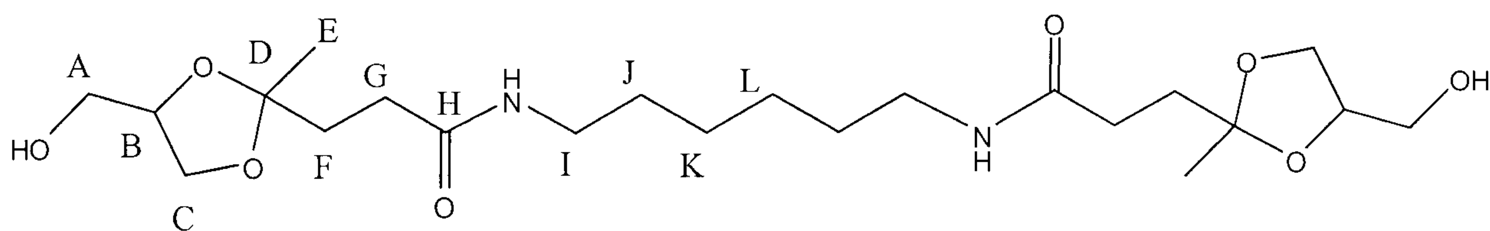
Carbon assignments
