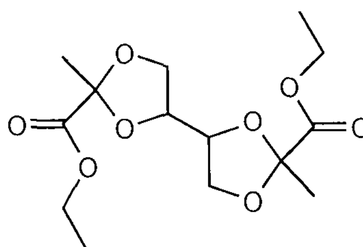
EtBPEK
