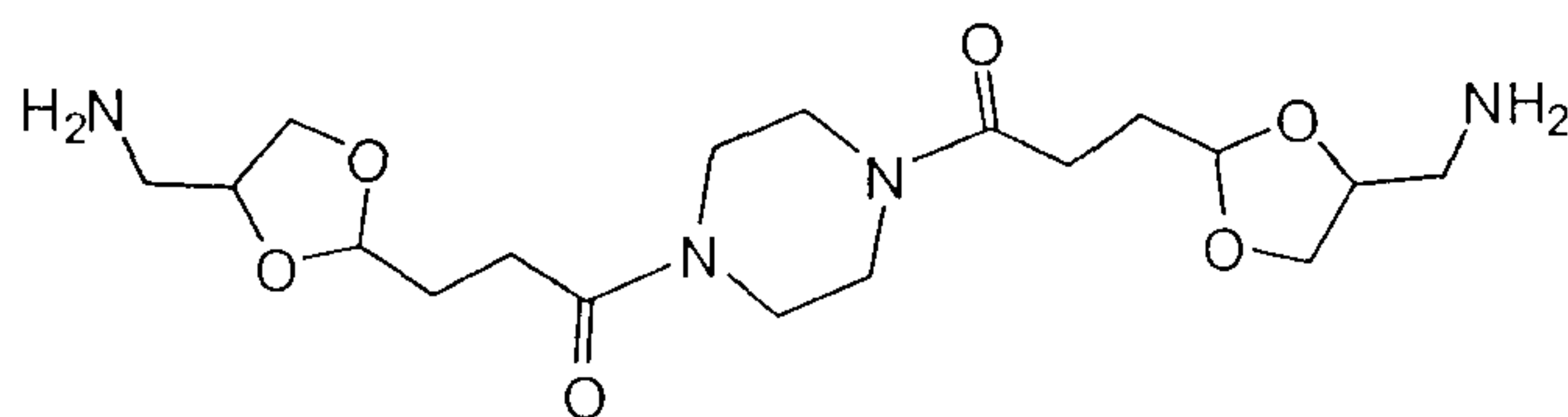
Ib
