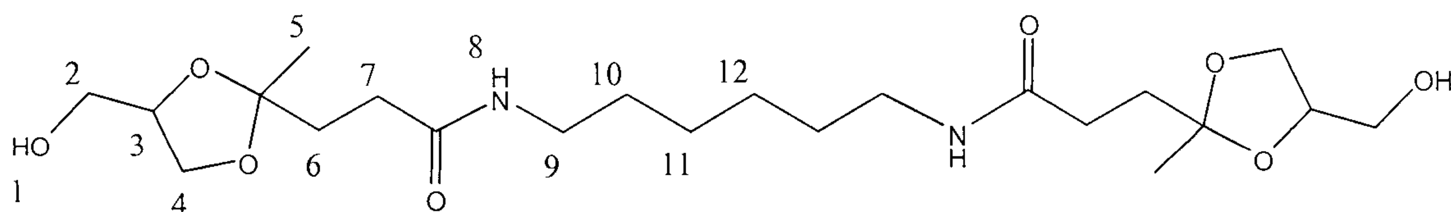
Proton assignments
