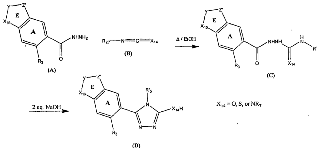
Scheme V: Synthesis of triazole compounds of the invention
